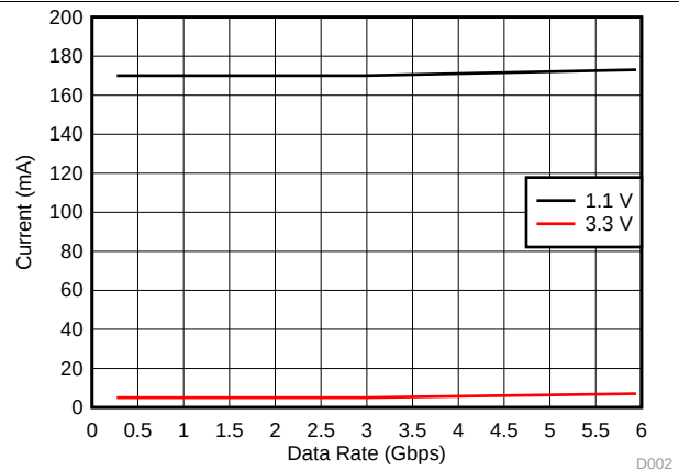
图 2. Current vs Data Rate in Redriver Mode
