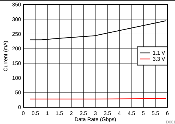
图 1. Current vs Data Rate in Retimer Mode
