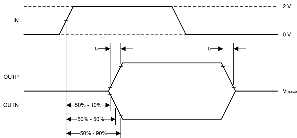
FIG 6-1. Rise, Fall, and Delay Time Definition
