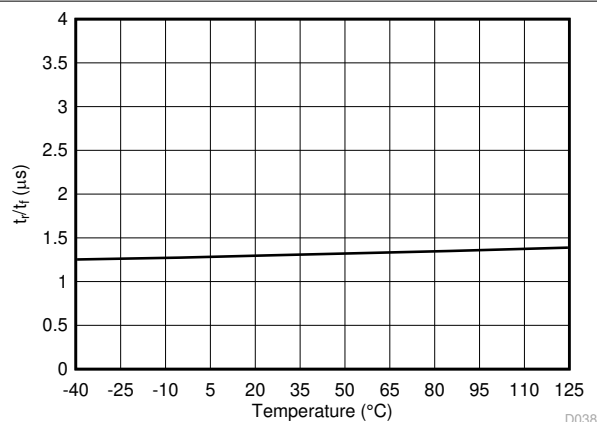
FIG 6-33. Output Rise and Fall Time vs Temperature
