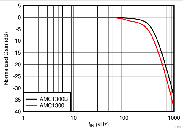
7-18. Normalized Gain vs Input Frequency
