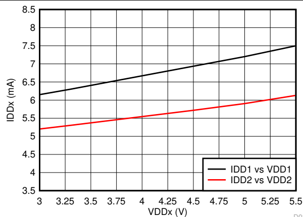
FIG 7-35. Supply Current vs Supply Voltage
