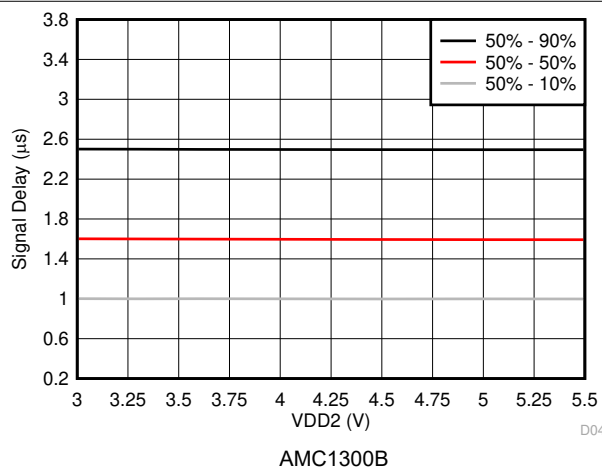
FIG 7-40. V IN to V OUT Signal Delay vs Low-Side Supply Voltage
