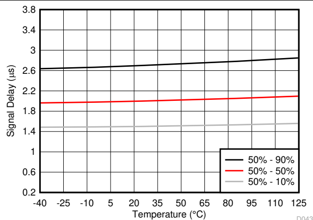
FIG 7-41. V_{IN} to V_{OUT} Signal Delay vs Temperature
