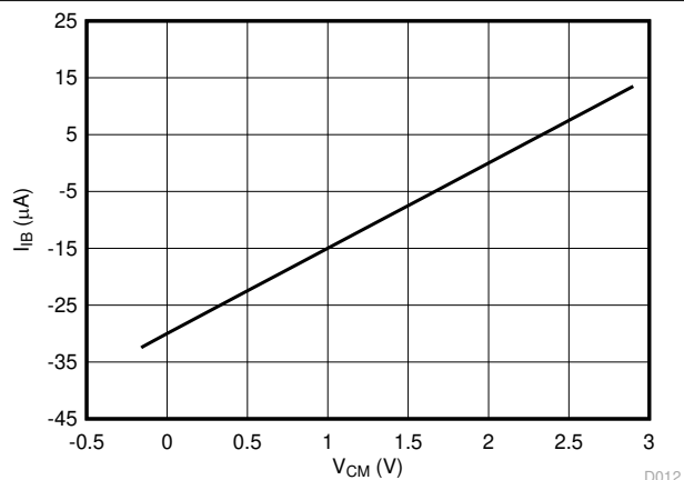
FIG 7-12. Input Bias Current vs Common-Mode Input Voltage
