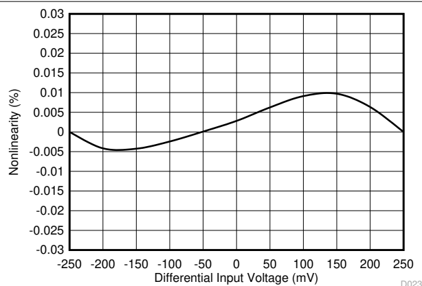
7-21. Nonlinearity vs Input Voltage
