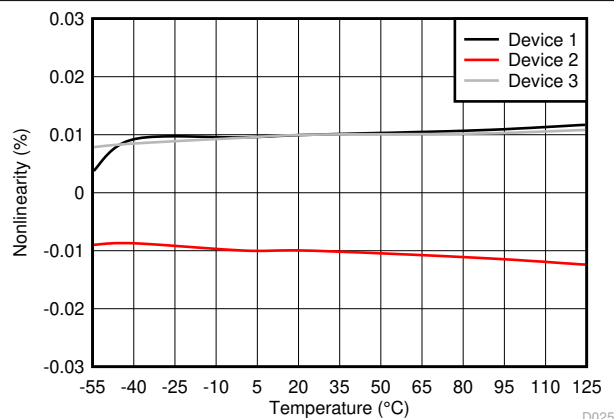
7-23. Nonlinearity vs Temperature
