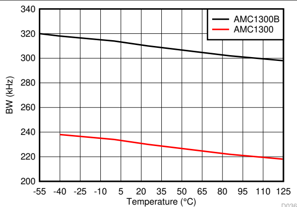
FIG 7-34. Output Bandwidth vs Temperature
