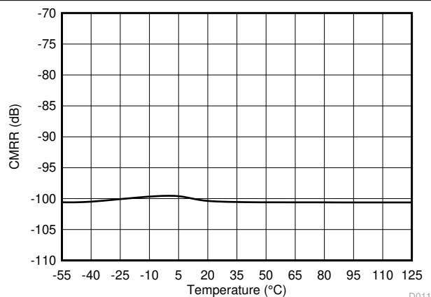
FIG 7-11. Common-Mode Rejection Ratio vs Temperature
