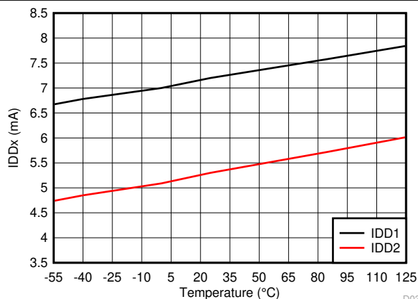
FIG 7-36. Supply Current vs Temperature
