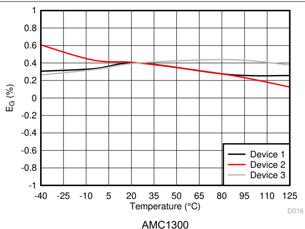
FIG 7-16. Gain Error vs Temperature
