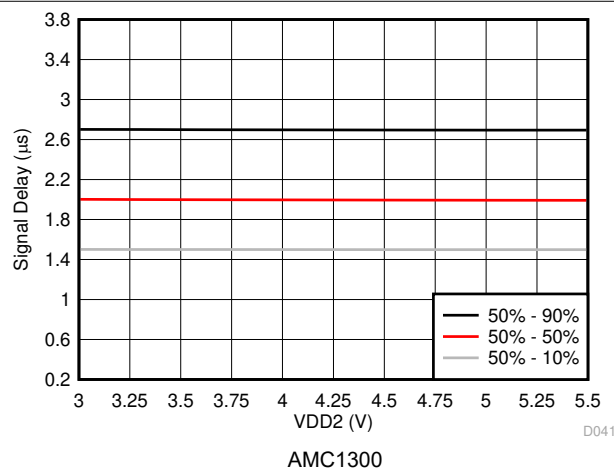
FIG 7-39. V IN to V OUT Signal Delay vs Low-Side Supply Voltage
