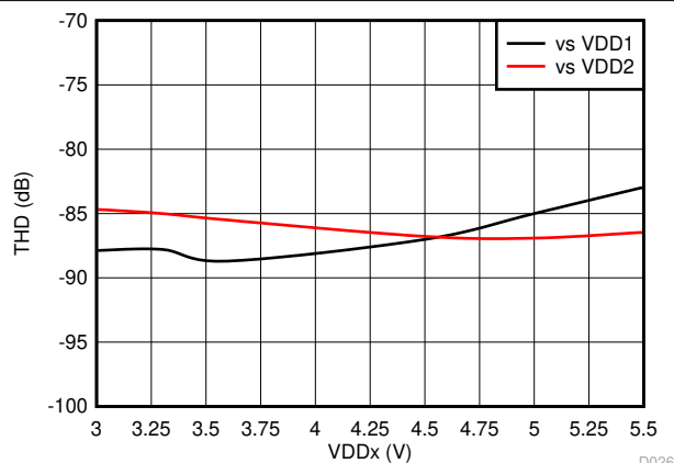
7-24. Total Harmonic Distortion vs Supply Voltage
