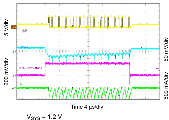
10-36. 1.2 V_{SYS} Load Transient, 0 to 200 mA
