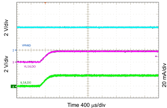
10-55. Startup Showing SS on LS/LDO in LDO Mode
