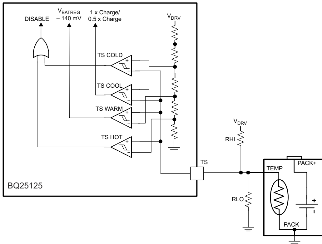
9-4. TS Circuit
