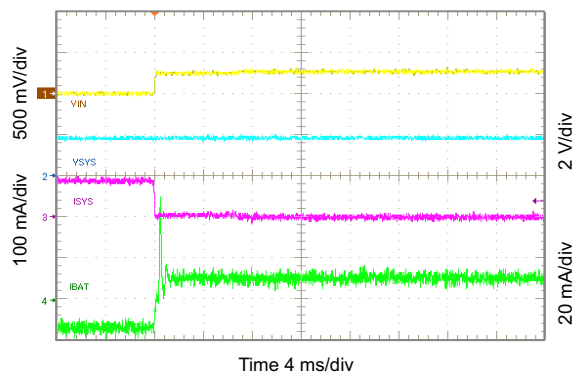
10-5. Exiting Battery Supplement Mode
