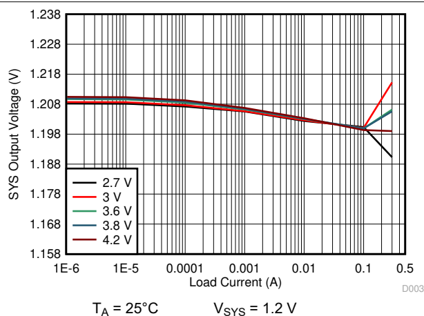
10-13. 1.2 V_{\text{SYS}} Load Regulation
