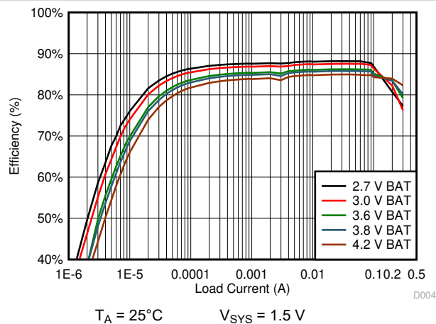
10-9. 1.5 V_{\text{SYS}} System Efficiency
