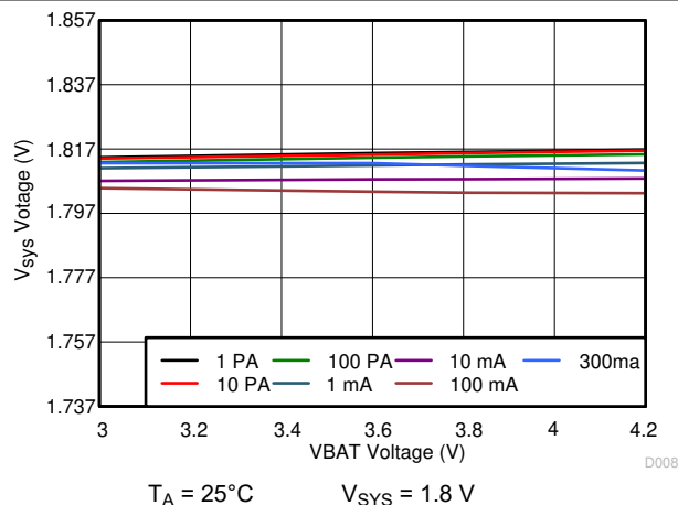
10-20. 1.8 V_{\text{SYS}} Line Regulation
