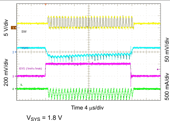
10-37. 1.8 V_{SYS} Load Transient, 0 to 200 mA
