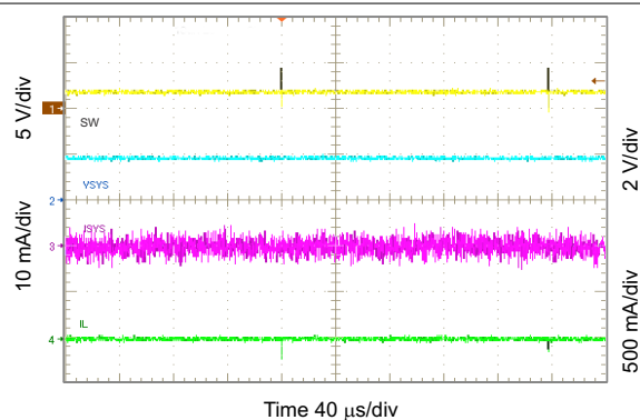
10-22. 3.3 V_{\text{SYS}} Line Regulation
