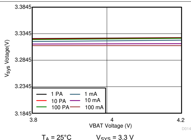
10-22. 3.3 V_{\text{SYS}} Line Regulation
