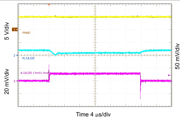
10-49. 3.3 V_{\text{LSLDO}} Load Transient, 0 to 10 mA
