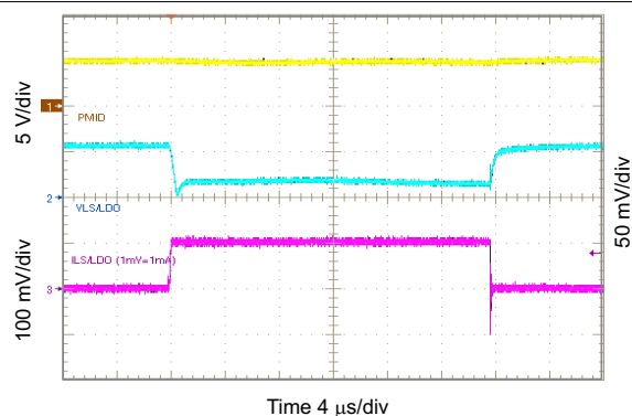
10-49. 3.3 V_{\text{LSLDO}} Load Transient, 0 to 10 mA
