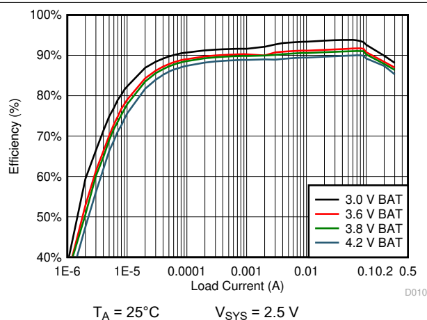
10-11. 2.5 V_{\text{SYS}} System Efficiency
