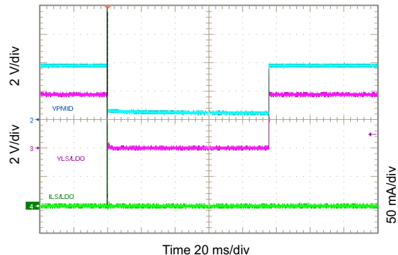
FIG 10-43. Short Circuit and Recovery for LS
