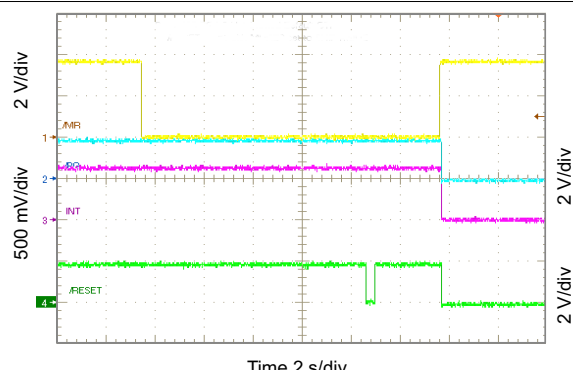
FIG 10-66. RESET Timing and Enter Ship Mode
