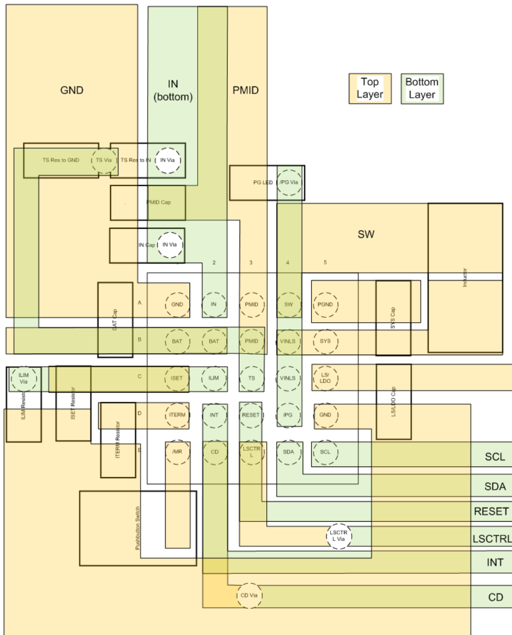
12-1. BQ25125 Layout
