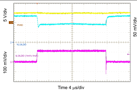
10-52. 1.8 V_{\text{LSLDO}} Load Transient, 0 to 100 mA
