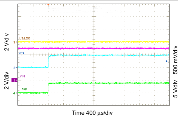
FIG 10-60. \overline{PG} Functions as Shifted \overline{MR} Output
