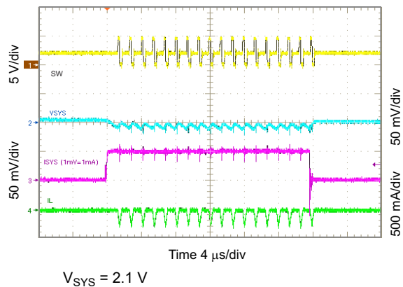
10-33. 2.1 V_{SYS} Load Transient, 0 to 50 mA
