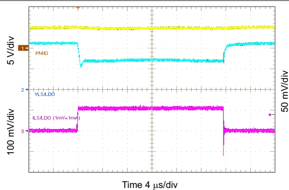
10-51. 1.2 V_{\text{LSLDO}} Load Transient, 0 to 100 mA
