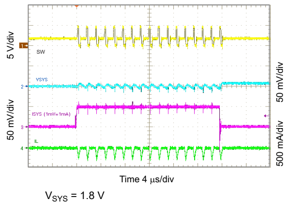
10-32. 1.8 V_{SYS} Load Transient, 0 to 50 mA
