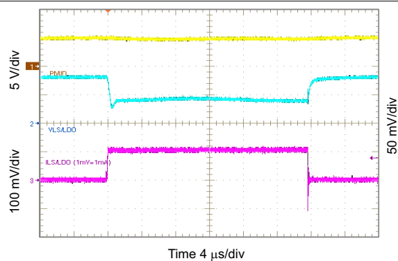
10-50. 0.8 V_{\text{LSLDO}} Load Transient, 0 to 100 mA
