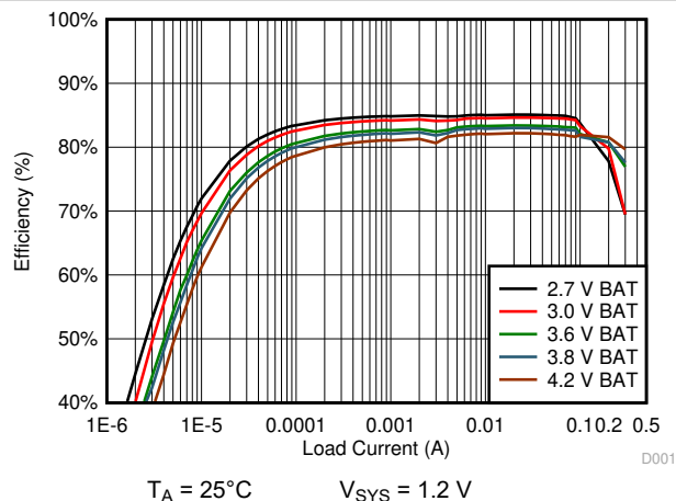
10-8. 1.2 V_{\text{SYS}} System Efficiency
