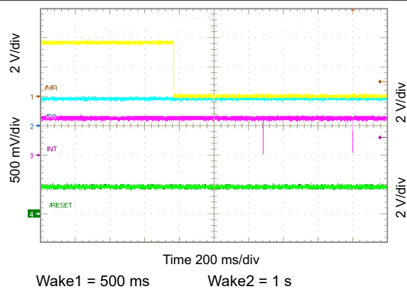
FIG 10-61. Show \overline{MR} Timing
