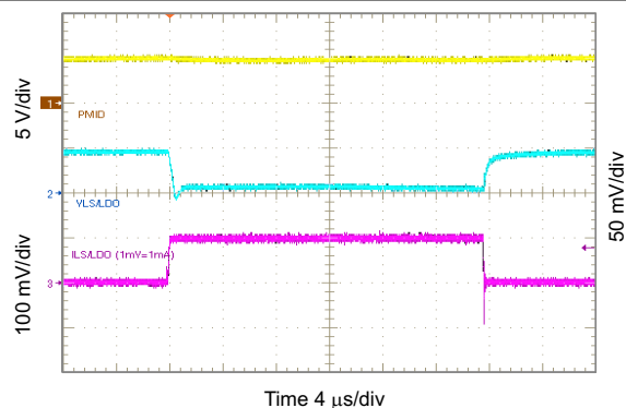
10-50. 0.8 V_{\text{LSLDO}} Load Transient, 0 to 100 mA
