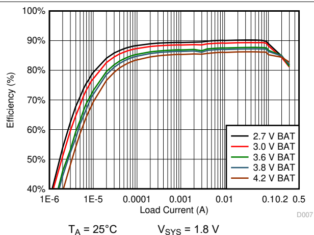
10-10. 1.8 V_{\text{SYS}} System Efficiency
