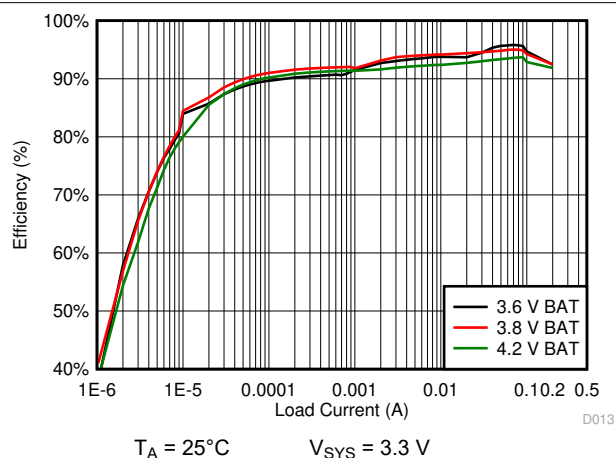
10-12. 3.3 V_{\text{SYS}} System Efficiency
