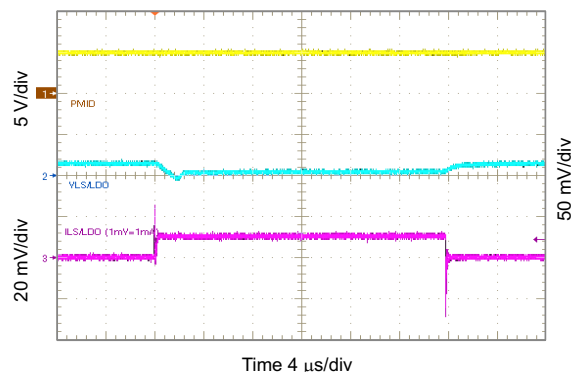
FIG 10-45. 0.8 V_{LSLDO} Load Transient, 0 to 10 mA
