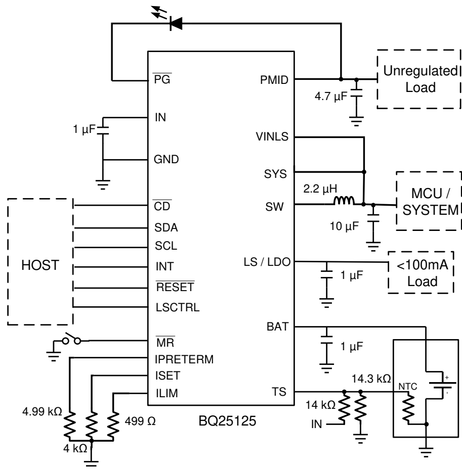
図 10-1. Typical Application Circuit
