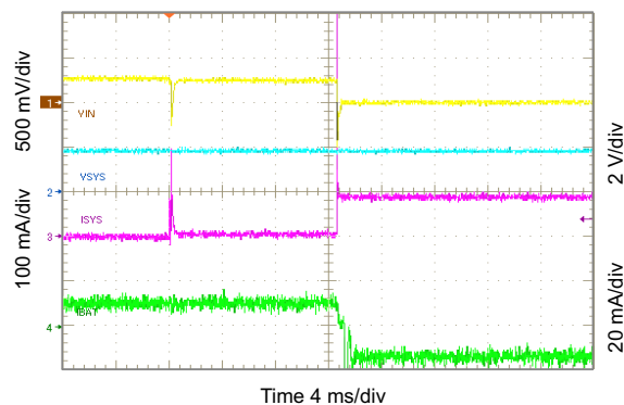
10-4. Entering Battery Supplement Mode
