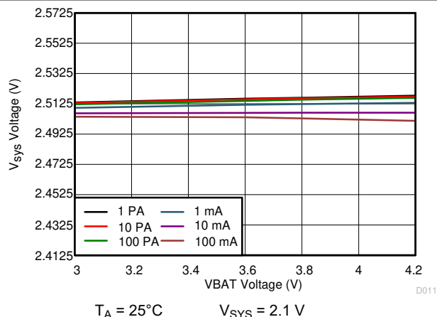
10-21. 2.1 V_{\text{SYS}} Line Regulation
