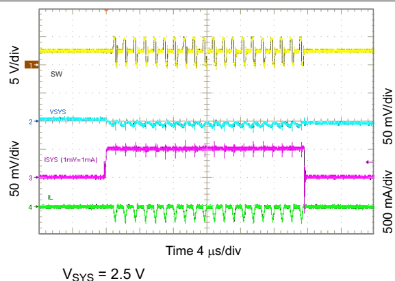
10-34. 2.5 V_{SYS} Load Transient, 0 to 50 mA
