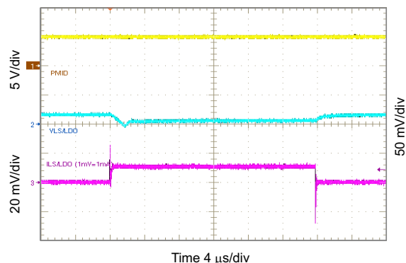
FIG 10-46. 1.2 V_{LSLDO} Load Transient, 0 to 10 mA
