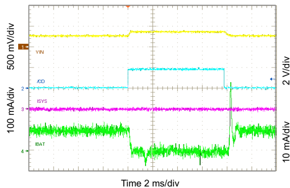
10-6. Charger On/Off Using \overline{CD}
