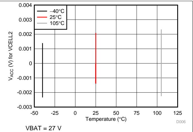
图 3. Total Channel Accuracy (V) for VCELL2
