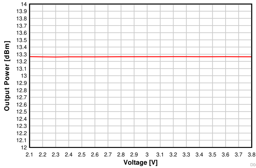
8-45. Output Power vs. Supply Voltage (VDD5) (50 kbps, 868.3 MHz)
