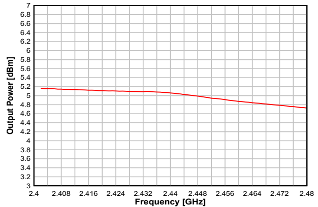
8-22. Output Power vs. Frequency (BLE 1 Mbps, 2.44 GHz, +5 dBm)
