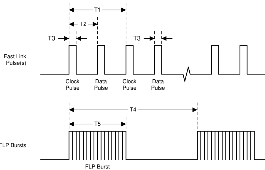
7-14. Fast Link Pulse Timing
