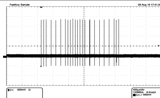
7-19. 10BASE-Tc Link Pulse Waveform
