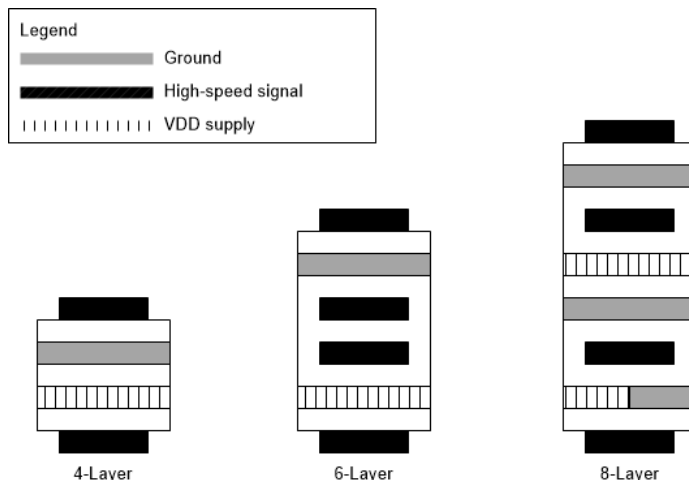
8-12. Recommended Layer Stack Up
