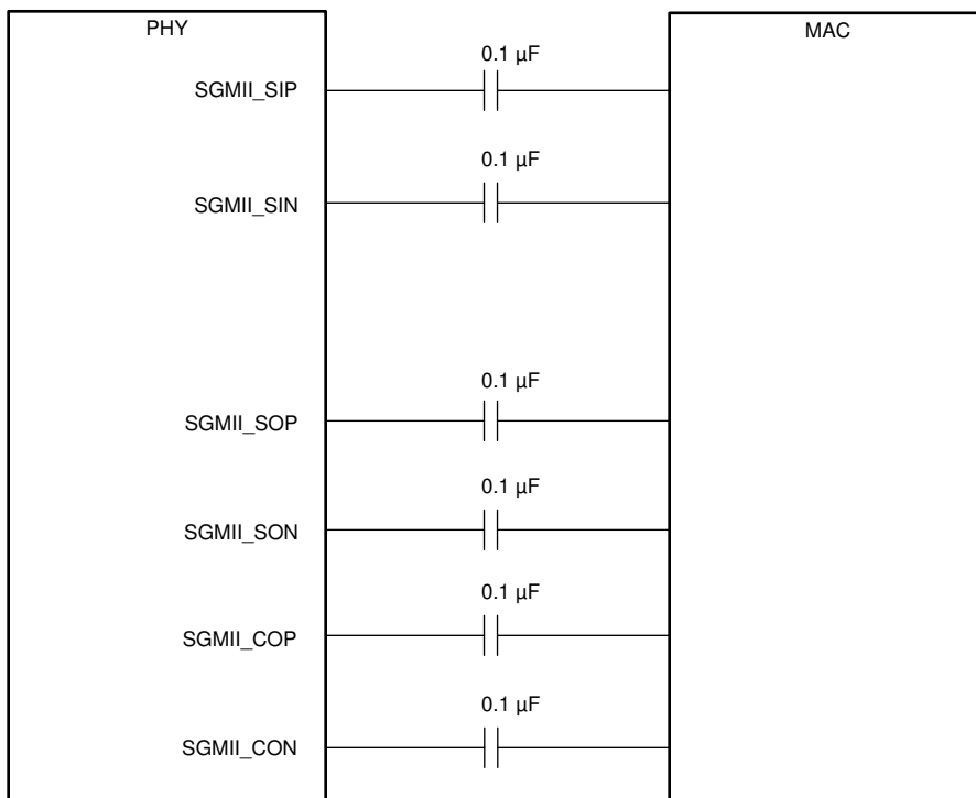
図 7-5. SGMII 6-Wire Connections
