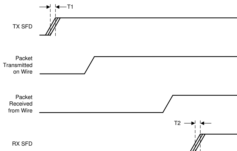
6-8. DP83867IS/CS Start of Frame Delimiter Timing
