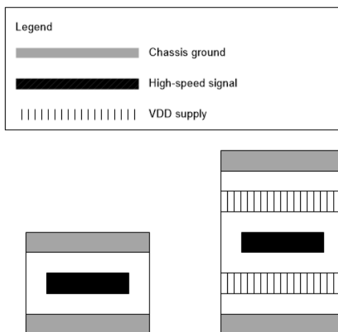
8-13. Alternative Layer Stack Up
