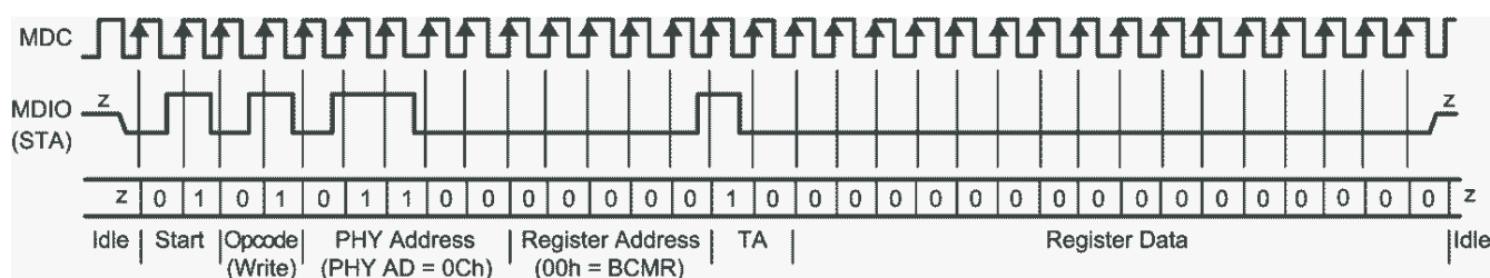
7-8. Typical MDC/MDIO Write Operation
