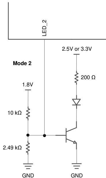
図 7-12. LED Operation From 1.8V I/O VDD Supply
