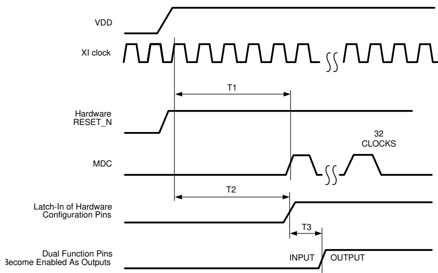
図 6-1. Power-Up Timing
