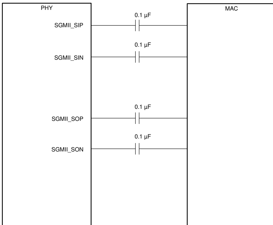
図 7-4. SGMII 4-Wire Connections
