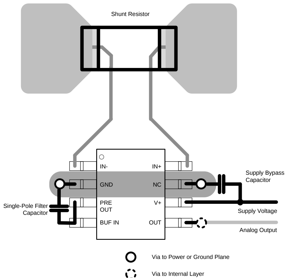
Figure 23. Example Layout
