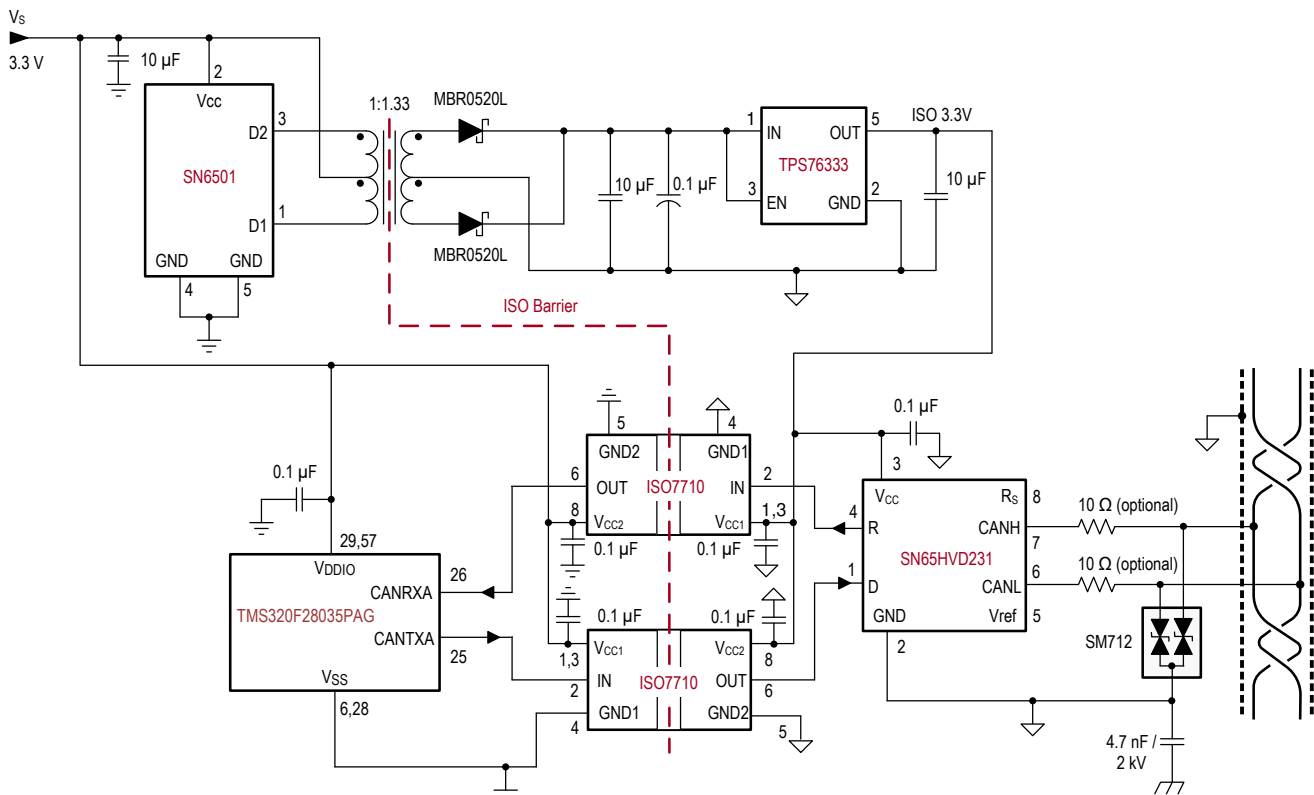
図 8-1. Isolated CAN Interface
