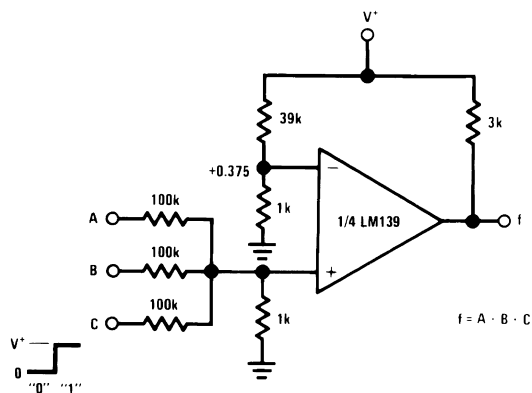
Figure 10. AND Gate ( V^+ = 5 V_{DC} )
