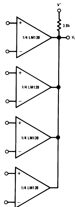
Figure 17. ORing the Outputs ( V_+ = 15\text{ V}_{\text{DC}} )
