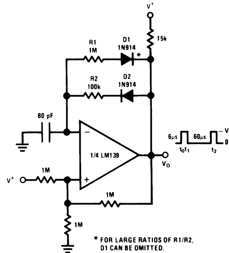
Figure 15. Pulse Generator ( V_+ = 15\text{ V}_{\text{DC}} )
