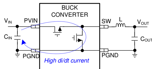
Figure 85. Buck Converter High di/dt Path
