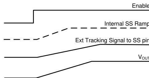
15. Tracking With Longer Start-up Time Than The Internal Ramp
