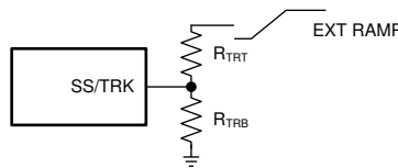
14. Soft-Start Tracking External Ramp
