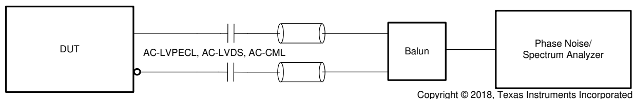
FIG 18. AC-LVPECL, AC-LVDS, AC-CML Output Phase Noise Test Configuration
