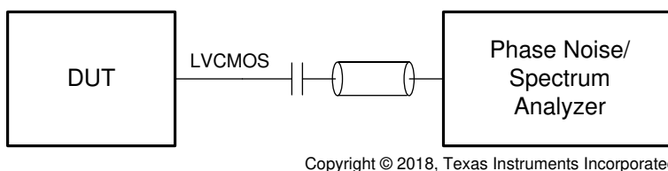
FIG 16. LVC MOS Output Phase Noise Test Configuration
