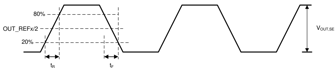
FIG 7-4. Single-Ended Output Voltage and Rise/Fall Time
