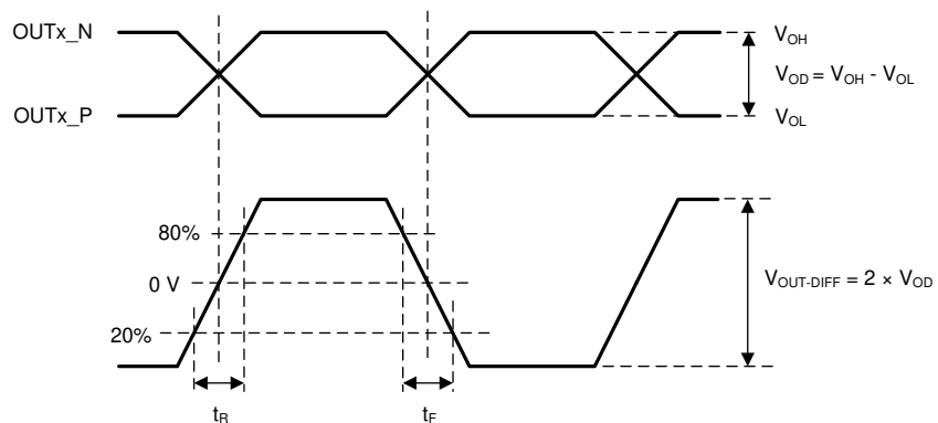
FIG 7-3. Differential Output Voltage and Rise/Fall Time
