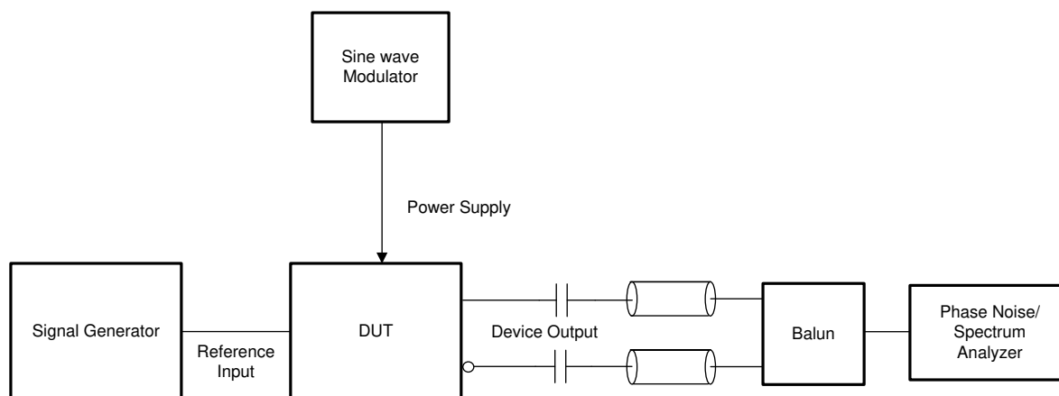
8-6. HCSL Output Phase Noise Test Configuration
