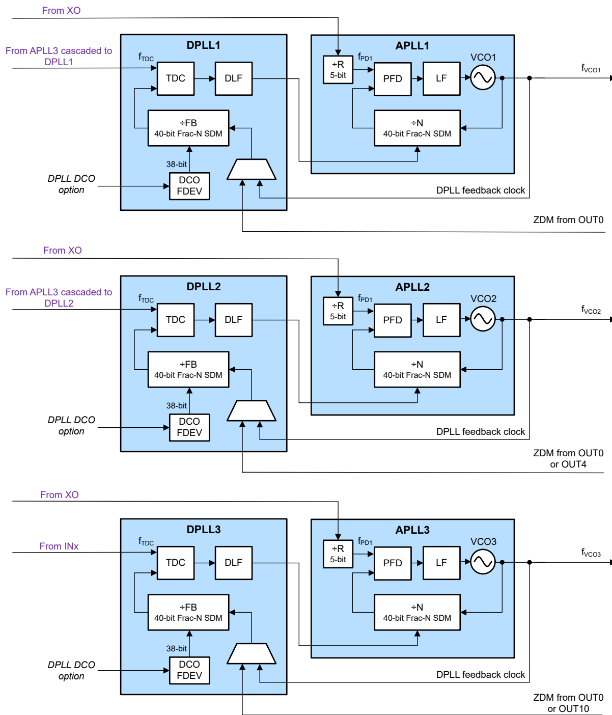
FIG 9-4. DPLL Cascaded Mode
