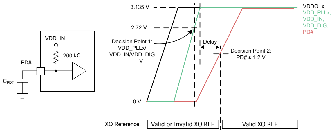
10-2. Recommendation for Power Up From Split-Supply Rails
