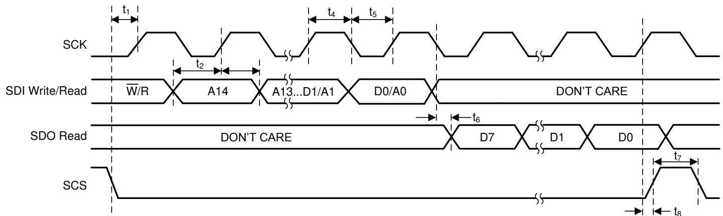
FIG 7-1. SPI Write Timing Diagram
