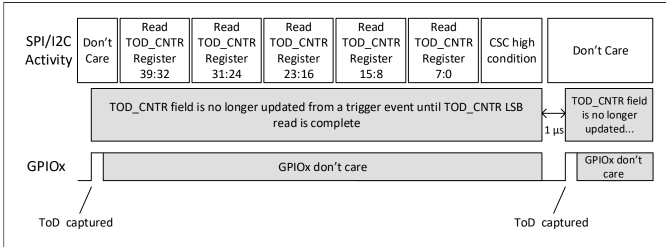
FIG 9-35. ToD Counter Captured Using GPIO1
