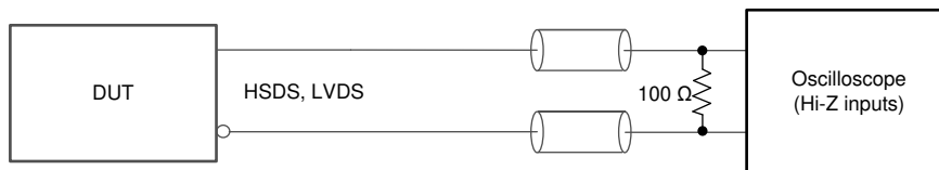
8-5. HSDS, LVDS Output DC Test Configuration
