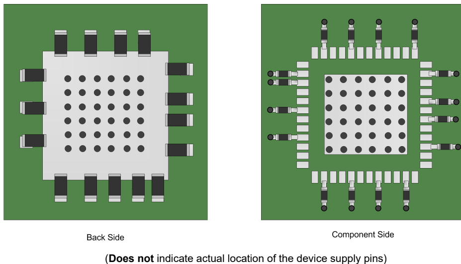
✕ 11-1. Generalized Placement of Power Supply Bypass Capacitors
