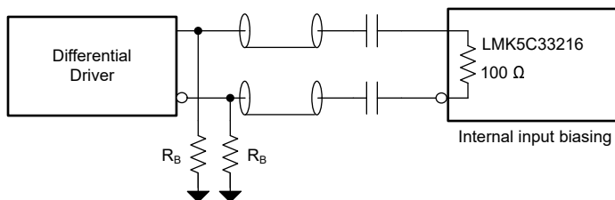
9-15. AC-Coupled Differential to Reference (INx)
