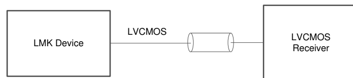
☒ 9-25. 1.8-V or 2.65-V LVCMOS Output to LVCMOS Receiver
