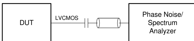
8-4. LVC MOS Output Phase Noise Test Configuration
