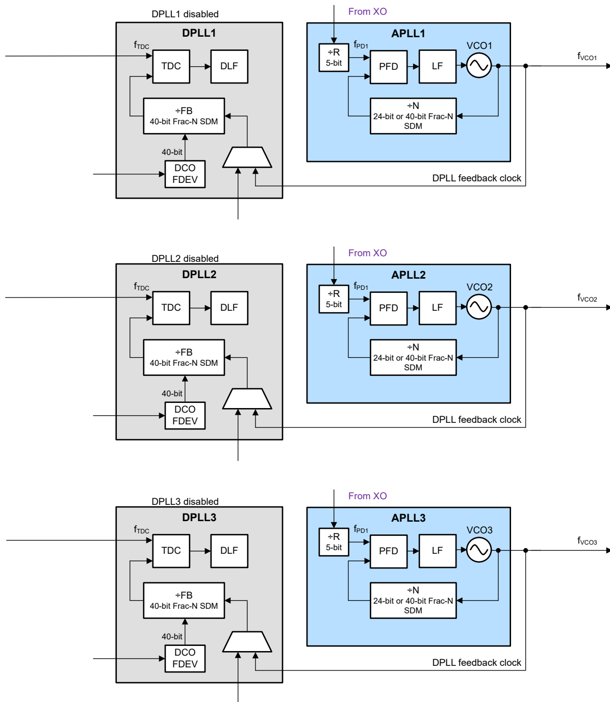
FIG 9-7. APLL-Only Independent Mode
