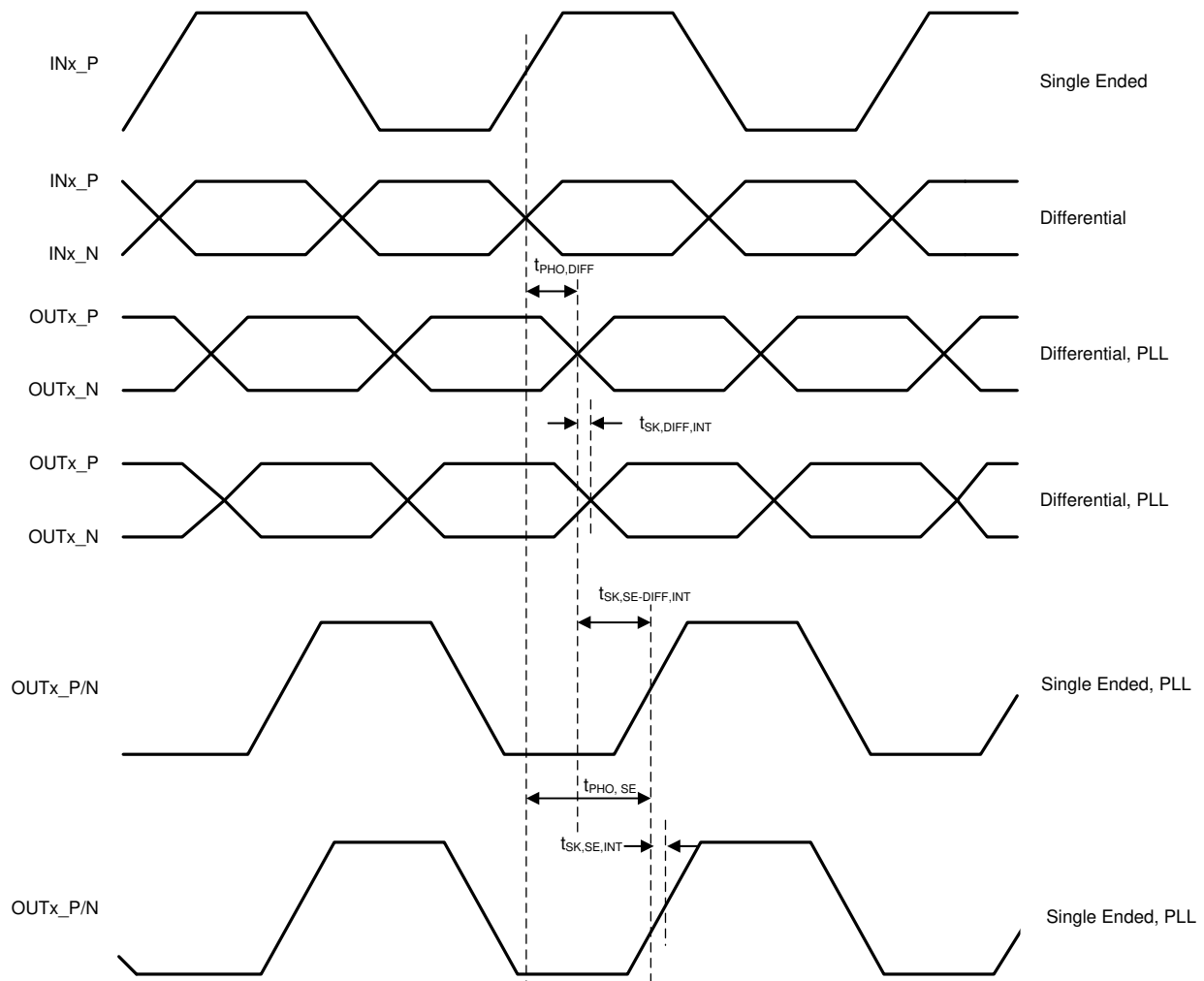
FIG 7-7. Differential and Single-Ended Output Skew and Phase Offset
