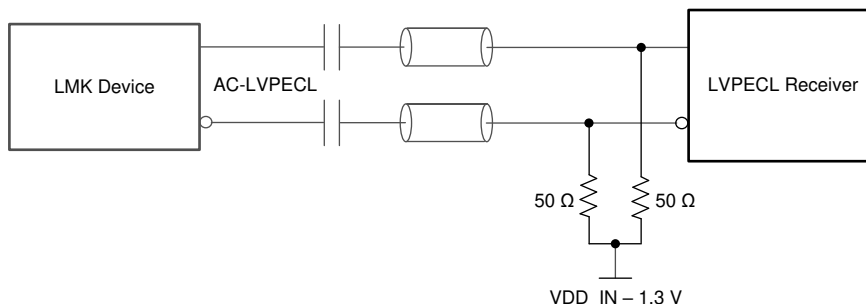
FIG 9-29. LVPECL Output AC coupling to LVPECL Receiver With External Termination/Biasing
