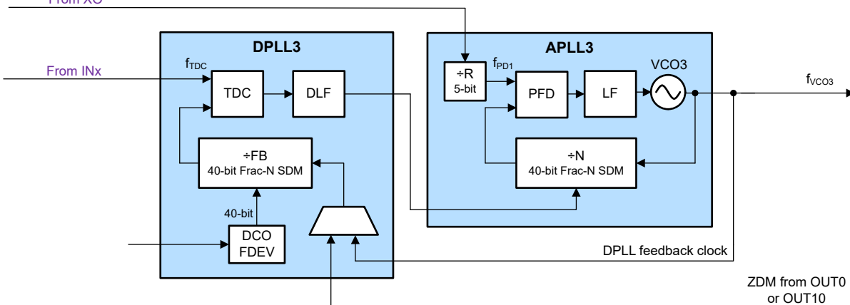
9-6. APLL Cascaded with DPLLs Disabled Example
