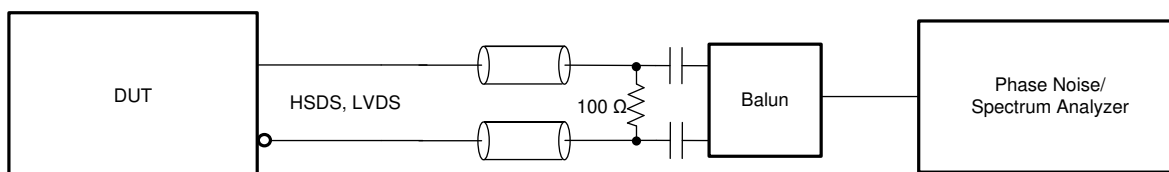
8-6. HSDS, LVDS Output Phase Noise Test Configuration
