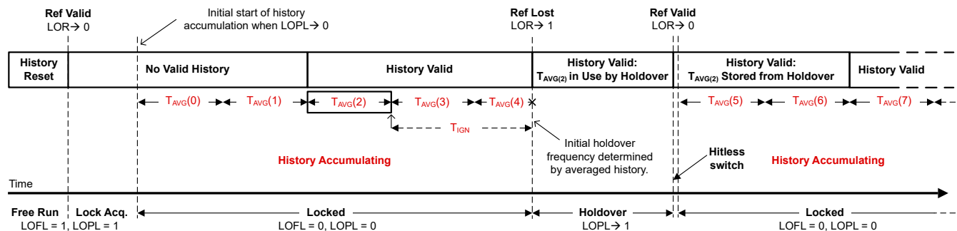
9-21. Tuning Word History Windows
