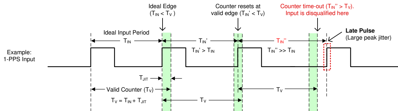
FIG 9-19. 1-PPS Input Window Detector Example
