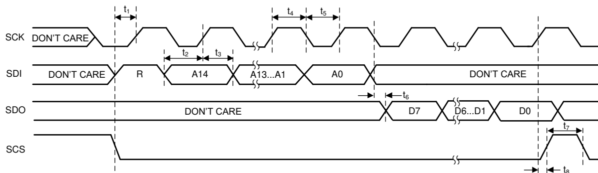
FIG 7-2. SPI 4-Wire Read Timing Diagram
