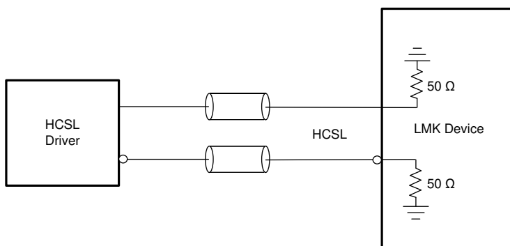
9-14. HCSSL (Load Terminated) to Reference (INx)
