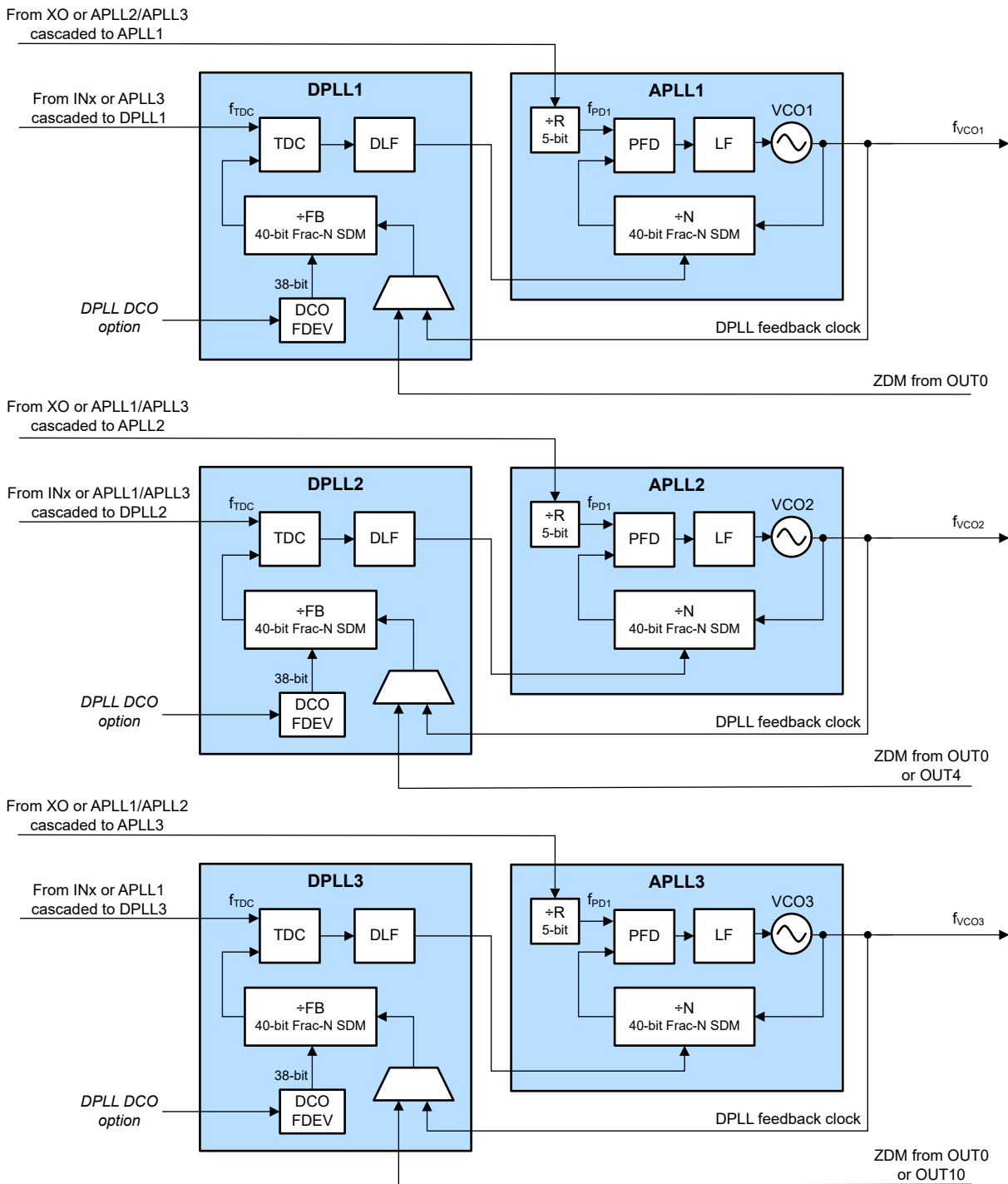
9-2. PLL Architecture
