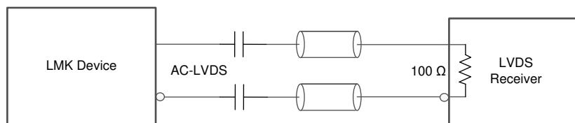
FIG 9-27. LVDS/HSDS Output AC coupling to LVDS Receiver with Internal Termination/Biasing
