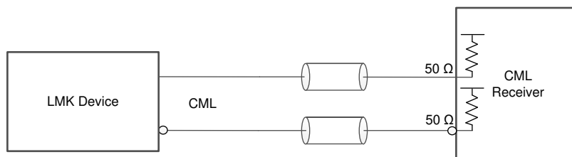
FIG 9-28. CML Open Collector Output to CML Receiver
