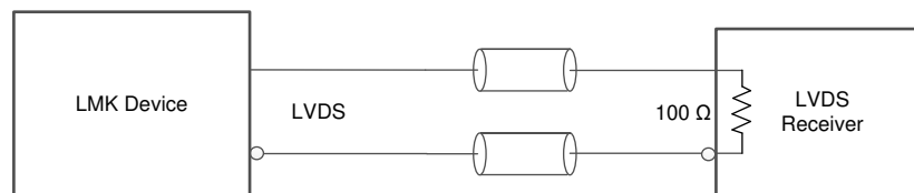
☒ 9-26. LVDS/HSDS Output DC coupling to LVDS Receiver
