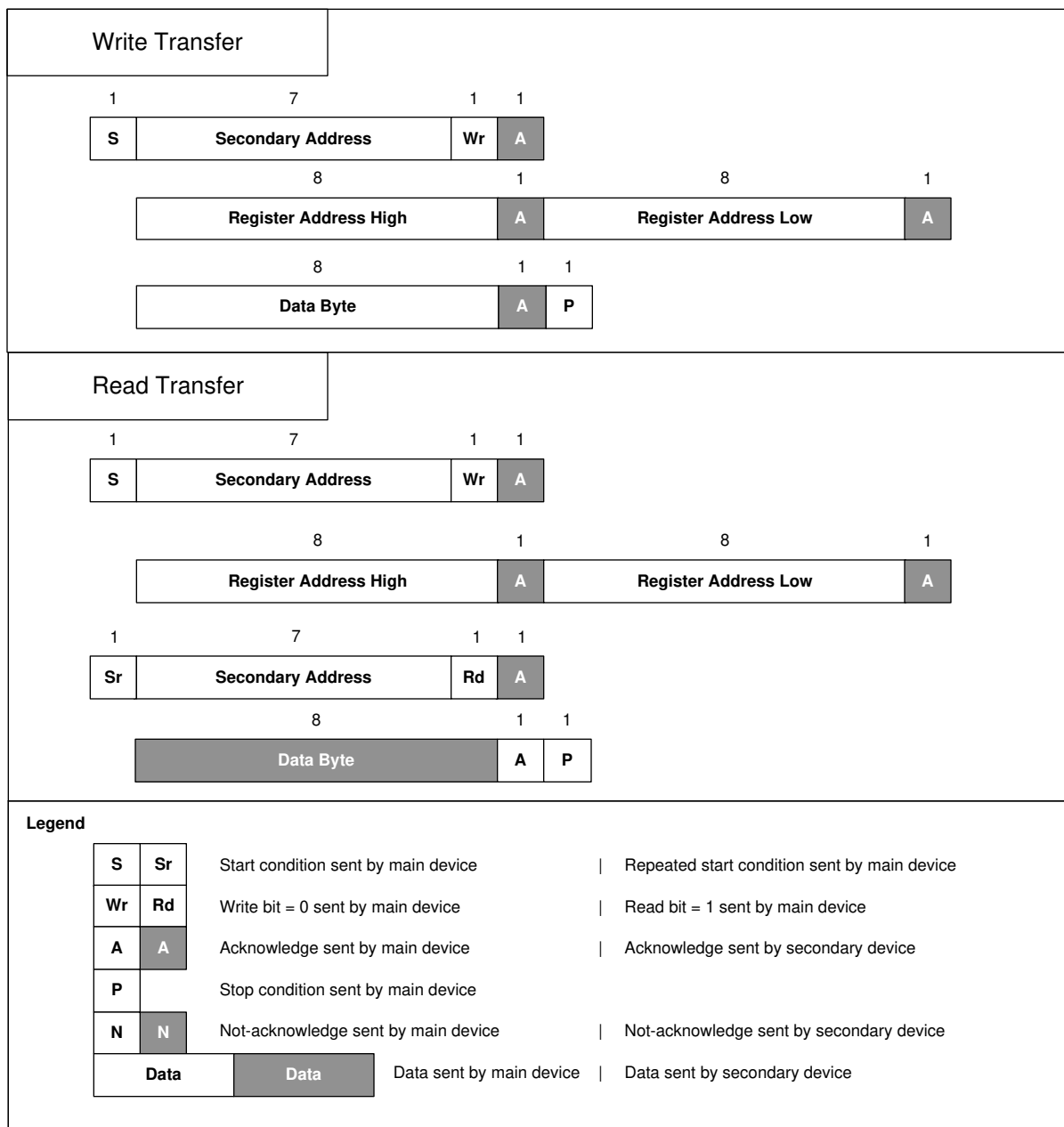
9-41. I 2 C Byte Write and Read Transfers
