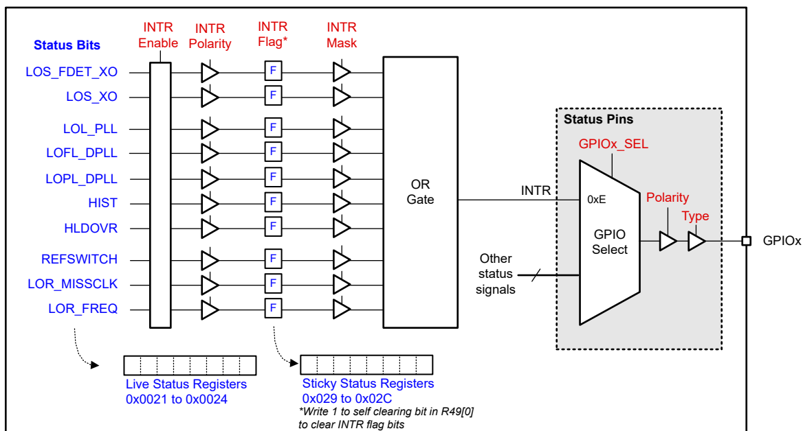
9-22. Status and Interrupt
