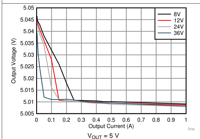
图 26. Line and Load Regulation
