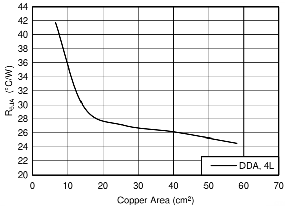
19. Typical R_{\theta JA} versus Copper Area for a Four-Layer Board and the HSOIC (DDA) Package
