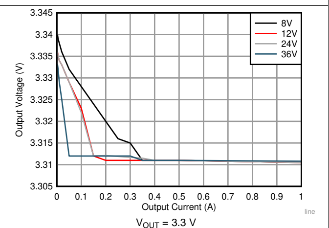
图 27. Line and Load Regulation
