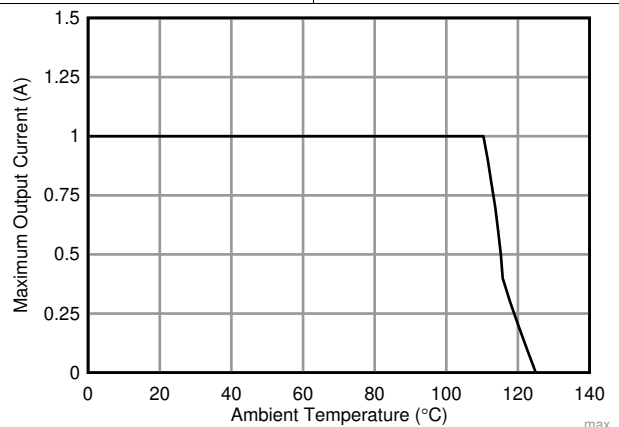
20. Maximum Output Current versus Ambient Temperature
