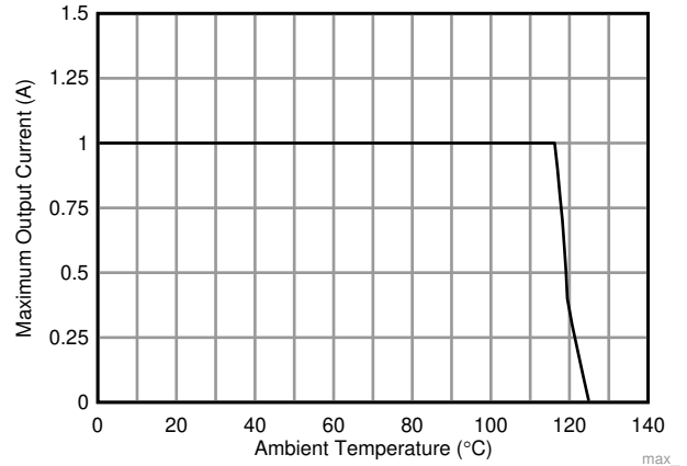
20. Maximum Output Current versus Ambient Temperature
