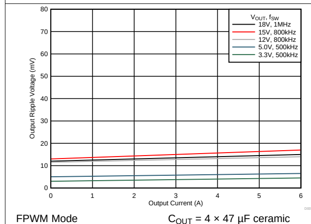
FIG 15. Output Voltage Ripple
