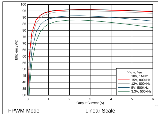
FIG 11. Efficiency vs Output Current
