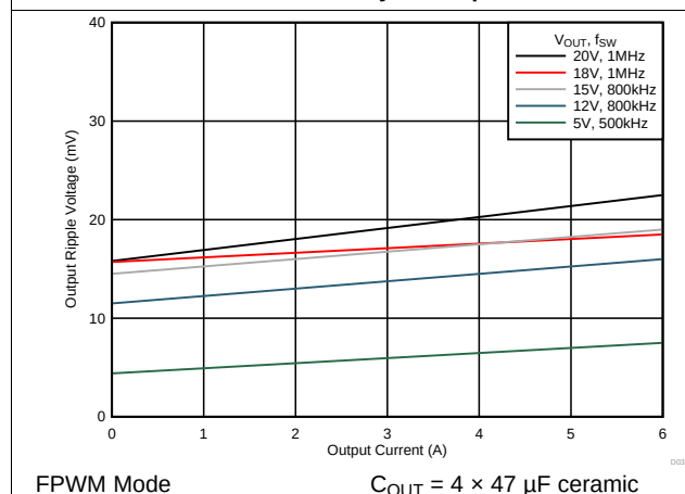
FIG 25. Voltage Ripple vs Output Current
