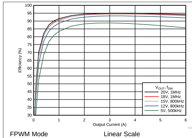
FIG 21. Efficiency vs Output Current
