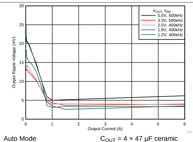
FIG 6. Voltage Ripple vs Output Current
