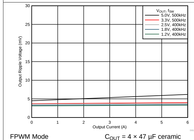
FIG 5. Voltage Ripple vs Output Current
