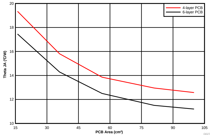
52. \theta_{JA} vs PCB Area
