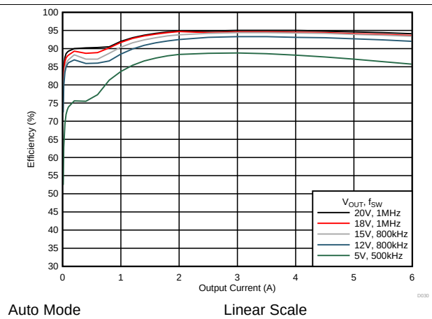
FIG 22. Efficiency vs Output Current
