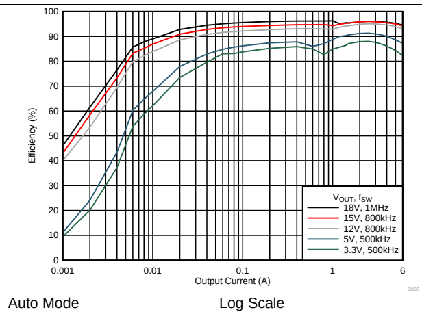
FIG 14. Efficiency vs Output Current
