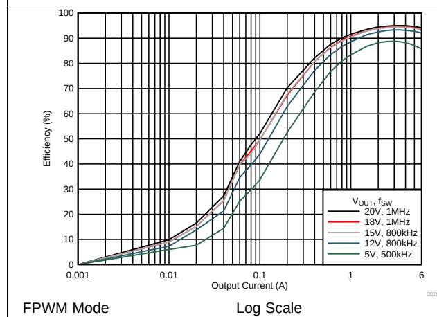
FIG 23. Efficiency vs Output Current
