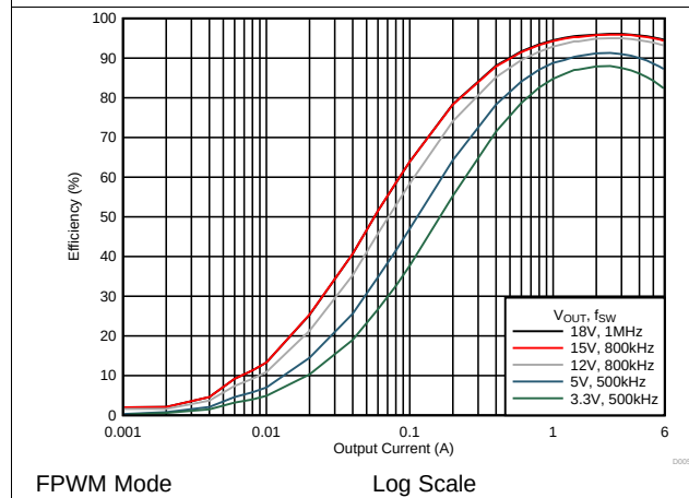
FIG 13. Efficiency vs Output Current
