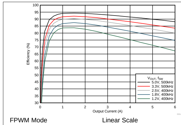
FIG 1. Efficiency vs Output Current
