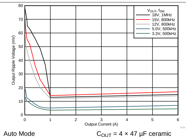
FIG 16. Output Voltage Ripple
