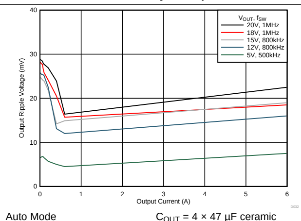
FIG 26. Voltage Ripple vs Output Current
