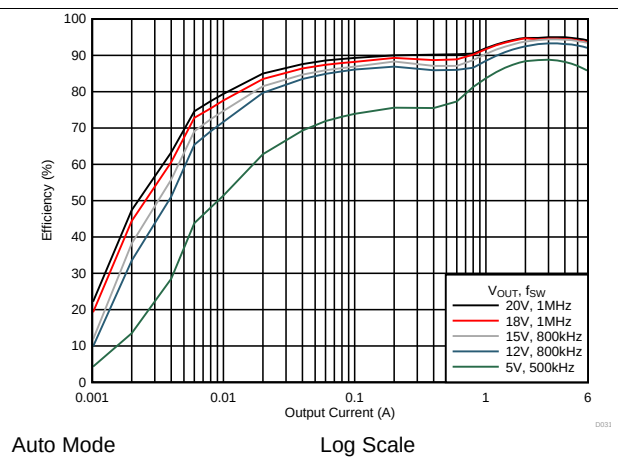
FIG 24. Efficiency vs Output Current
