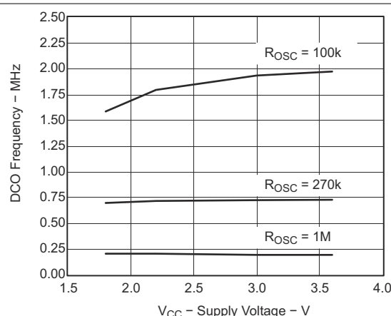
8-22. DCO Frequency vs Supply Voltage (T A = 25°C)
