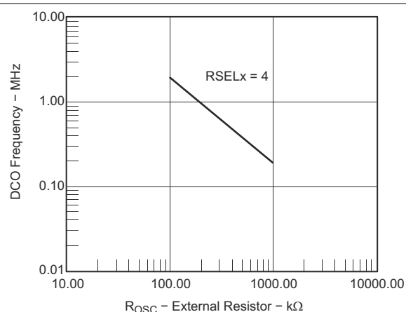
8-20. DCO Frequency vs R_{OSC} (V CC = 3 V, T A = 25°C)
