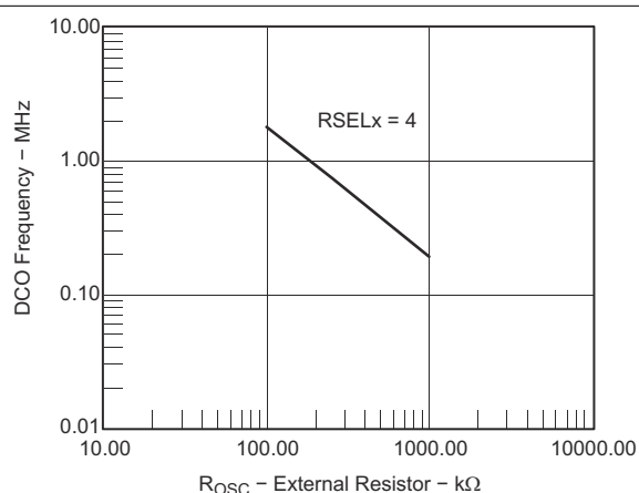
8-19. DCO Frequency vs R_{OSC} (V CC = 2.2 V, T A = 25°C)
