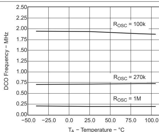
8-21. DCO Frequency vs Temperature (V CC = 3 V)
