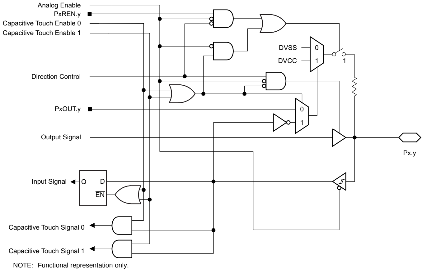
☒ 6-2. Capacitive Touch I/O Functionality
