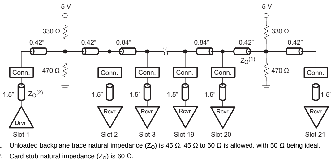
Figure 6. VME64x Backplane
