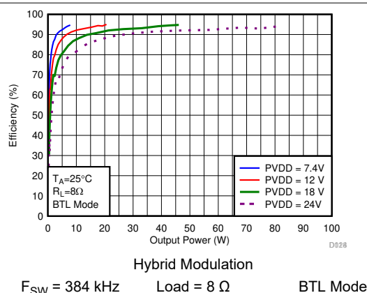
Figure 7-22. Efficiency vs Output Power
