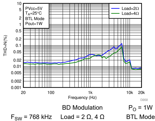
Figure 7-36. THD+N vs Frequency-BTL
