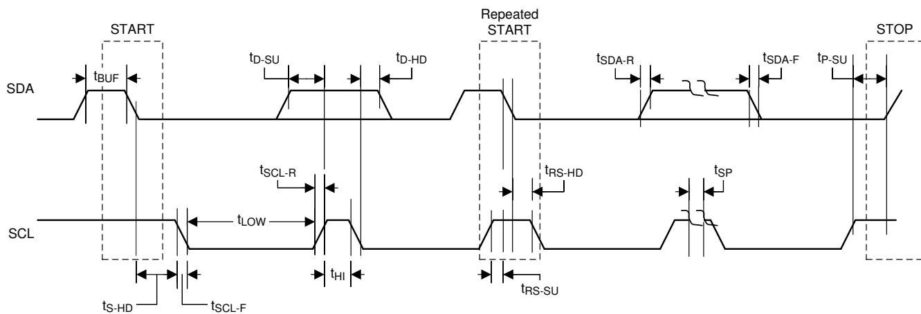
FIG 8-2. I²C Communication Port Timing Diagram
