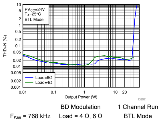
7-54. THD+N vs Output Power-BTL
