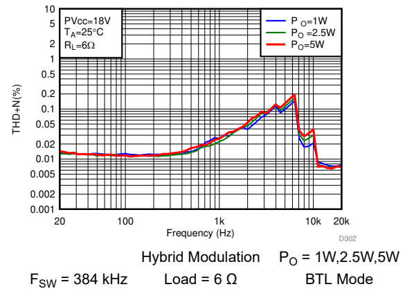
FIG 7-8. THD+N vs Frequency-BTL
