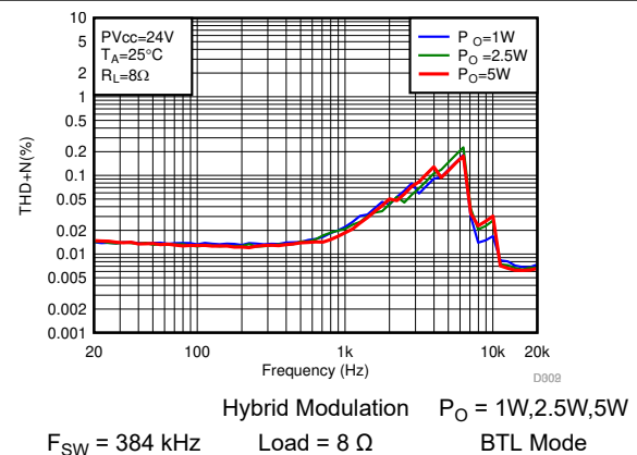
FIG 7-10. THD+N vs Frequency-BTL
