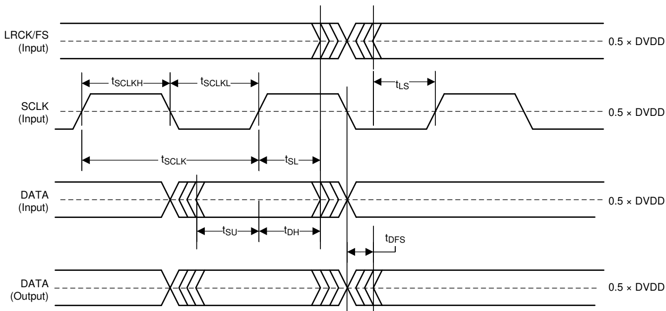
FIG 8-1. Serial Audio Port Timing in Target Mode
