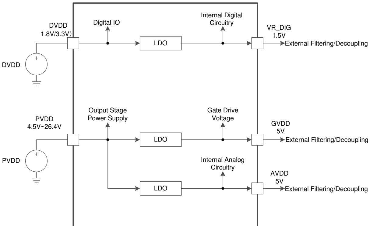
FIG 10-12. Power Supply Function Block Diagram
