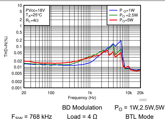
Figure 7-43. THD+N vs Frequency-BTL
