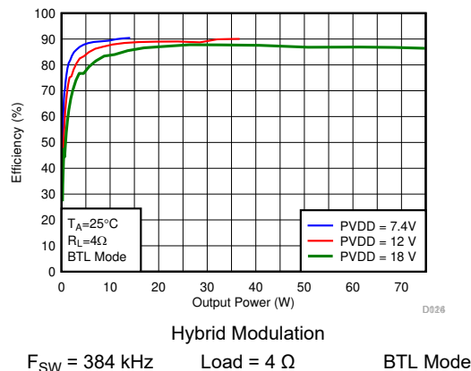
Figure 7-20. Efficiency vs Output Power
