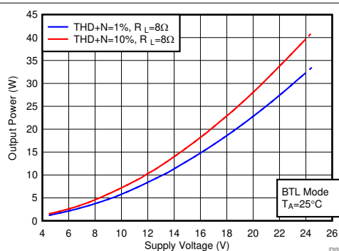
7-55. Output Power vs Supply Voltage
