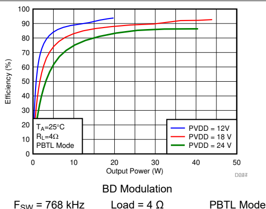
7-76. Efficiency vs Output Power
