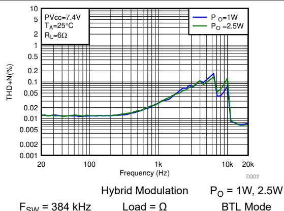
Figure 7-2. THD+N vs Frequency-BTL
