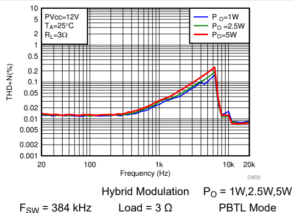
Figure 7-24. THD+N vs Frequency-PBTL
