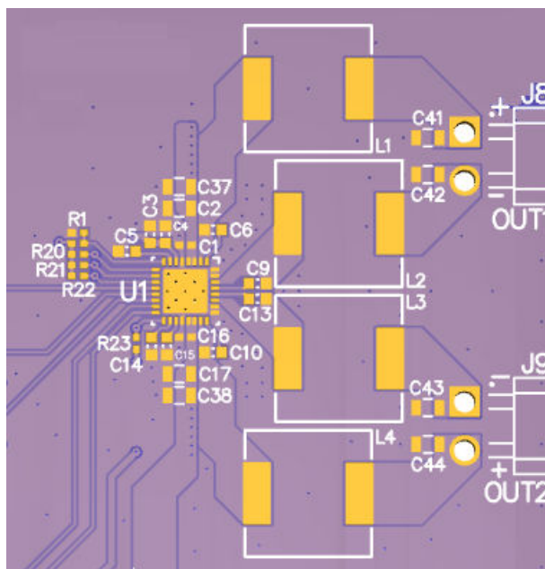
10-14. 2.0 (Stereo BTL) Top Copper View
