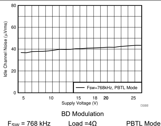
7-77. Idle Channel Noise vs Supply Voltage
