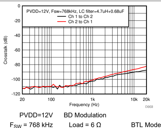
7-59. Crosstalk
