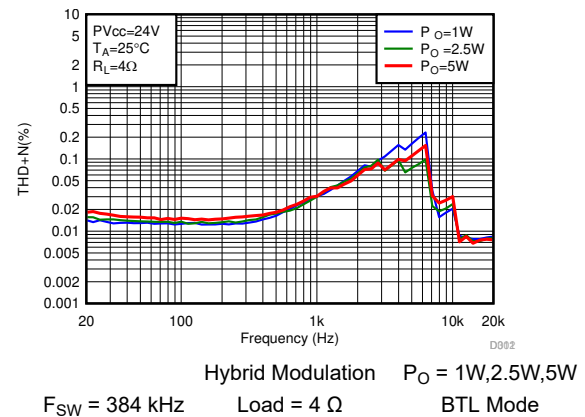
FIG 7-12. THD+N vs Frequency-BTL
