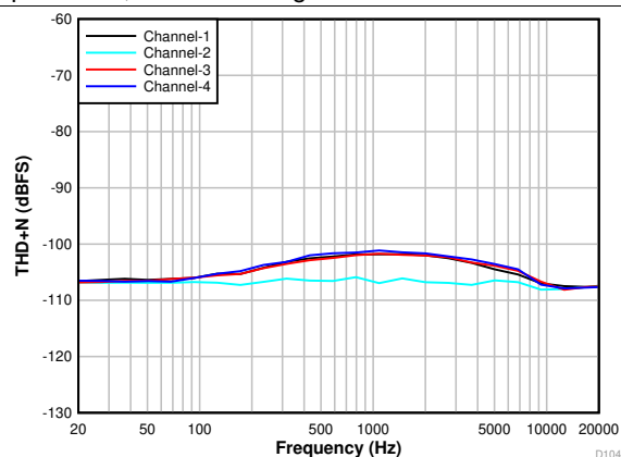
FIG 12. THD+N vs Input Frequency With a -1-dBr Input
