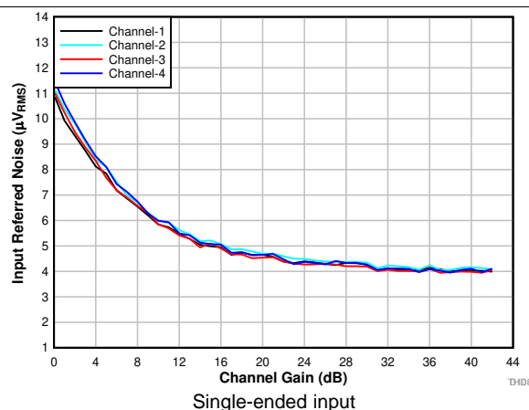
FIG 14. Input-Referred Noise vs Channel Gain Single-ended input
