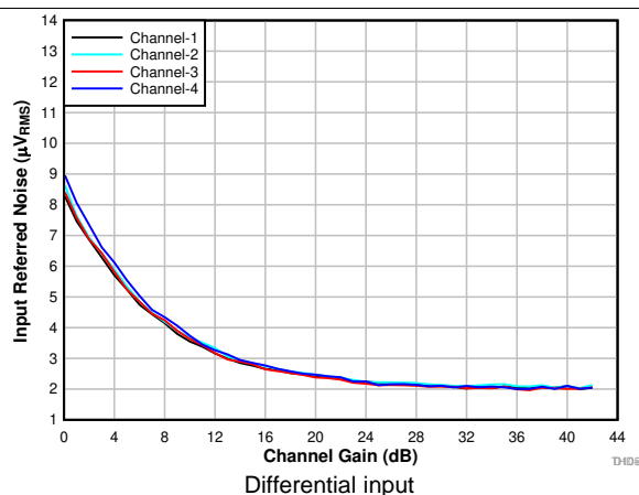
FIG 13. Input-Referred Noise vs Channel Gain Differential input
