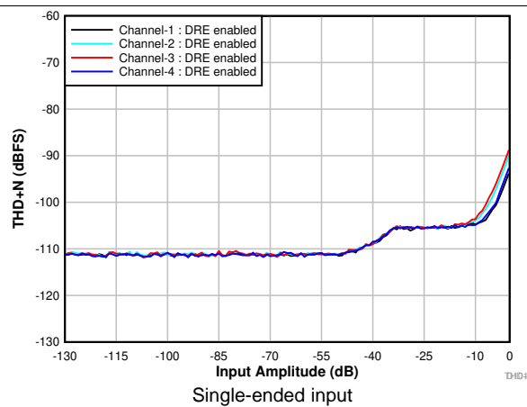
Figure 7. THD+N vs Input Amplitude With DRE Enabled
