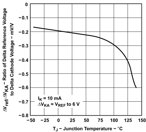
図 5-9. Ratio of Delta Reference Voltage to Delta Cathode Voltage vs Junction Temperature (for TLV431 and TLV431A)
