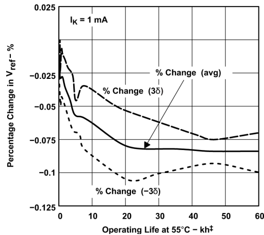
図 5-11. Percentage Change in v_{REF} vs Operating Life at 55°C
