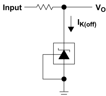
6-3. Test Circuit for I_{K(off)}
