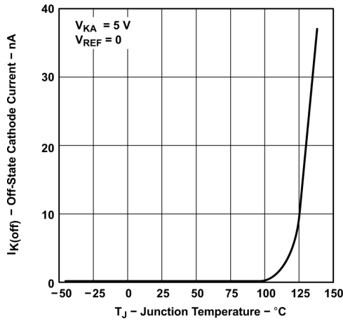
図 5-7. Off-State Cathode Current vs Junction Temperature (for TLV431 and TLV431A)
