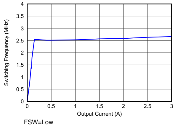
Figure 23. Switching Frequency
