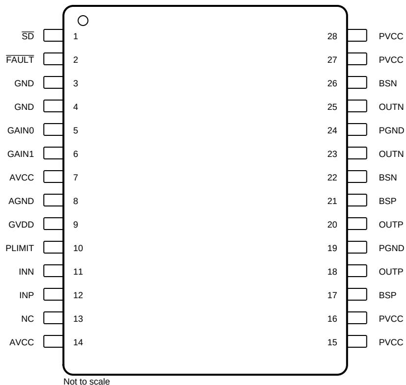
Pin Functions
