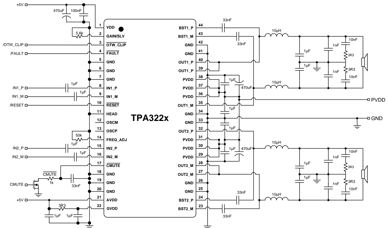
✎ 50. Typical Differential (2N) AD-Mode BTL Application
