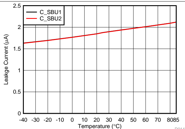
図 8. SBU Path Leakage Current vs Ambient Temperature at 3.6 V
