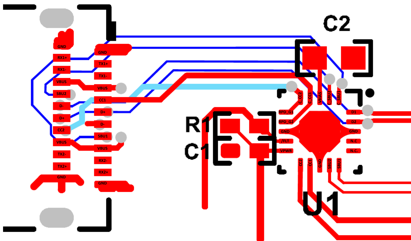
34. TPD6S300A Typical Layout
