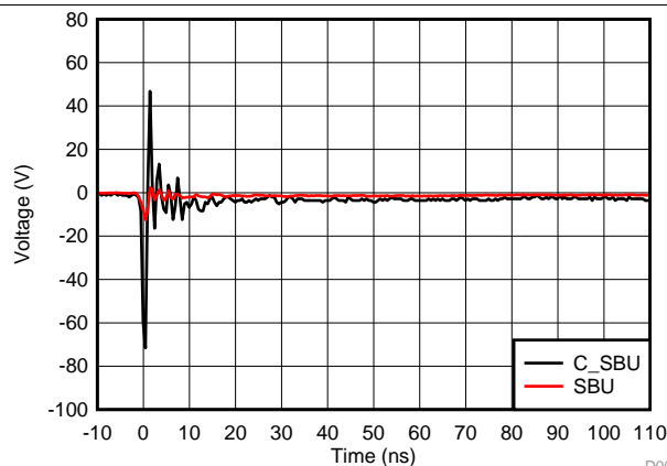
図 7. SBU IEC 61000-4-2 -4-kV Response Waveform
