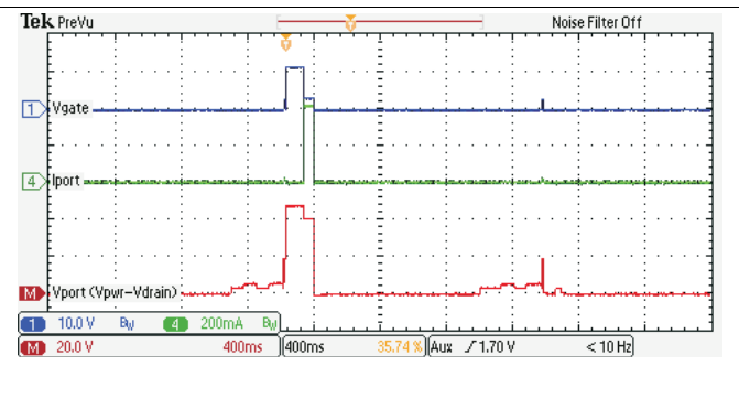
Figure 32. Current Limit 15-ms Timeout: PoE+ Mode, 45-Ω Load
