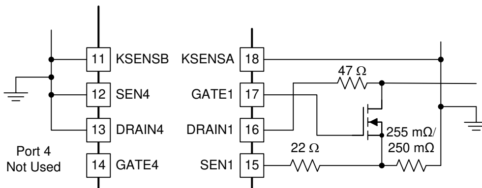
Figure 47. Unused PORT4 Connections
