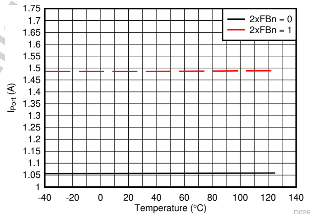
7-24. I SHORT Threshold vs Temperature
