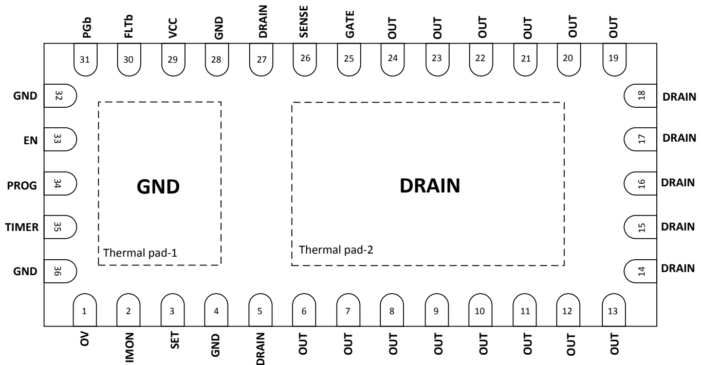
Pin Functions
