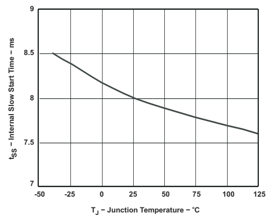
图 5-6. Internal Slow-Start Time vs Junction Temperature
