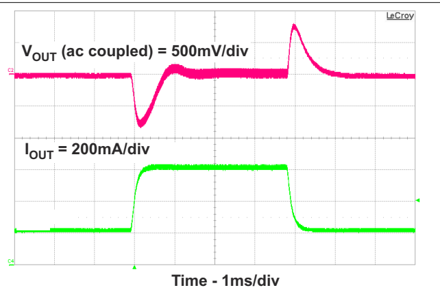
8-4. Load Transient Response
