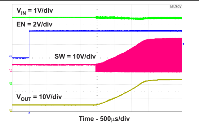
8-8. Start-Up
