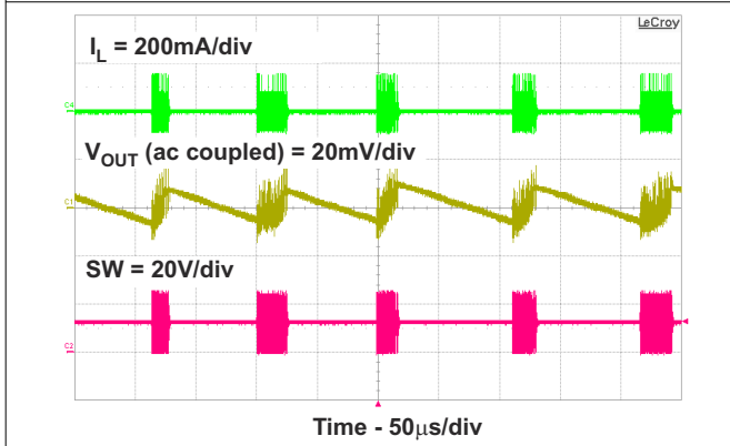
8-7. Pulse Skipping
