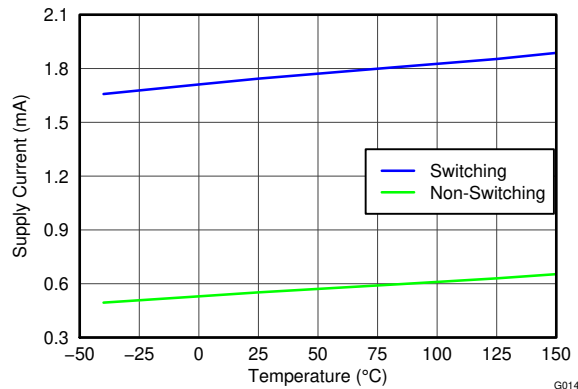
6-15. Supply Current vs Temperature
