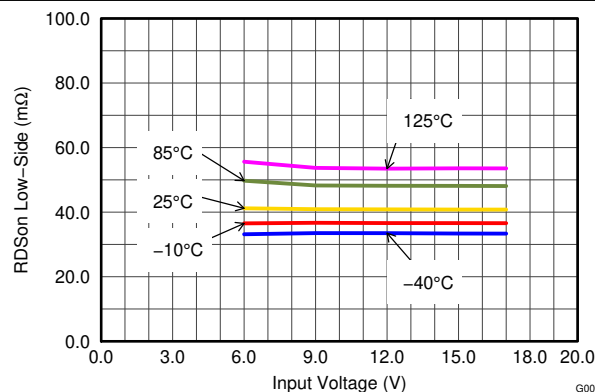
7-4. Low-Side Switch Resistance
