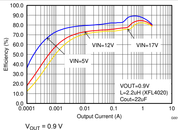
9-14. Efficiency With 1.25 MHz
