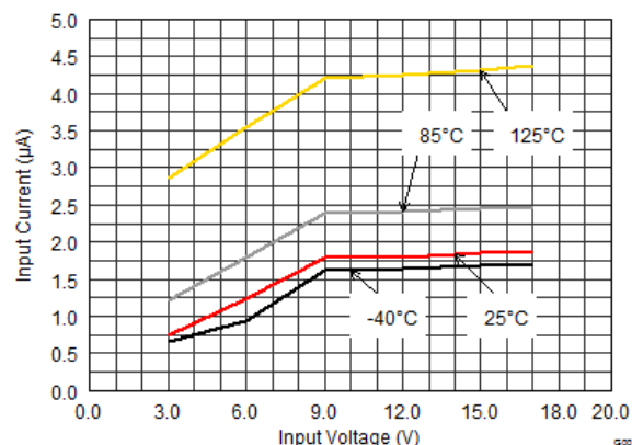
7-2. Shutdown Current
