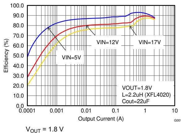
9-12. Efficiency With 1.25 MHz
