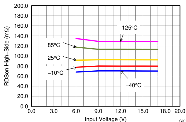
7-3. High-Side Switch Resistance
