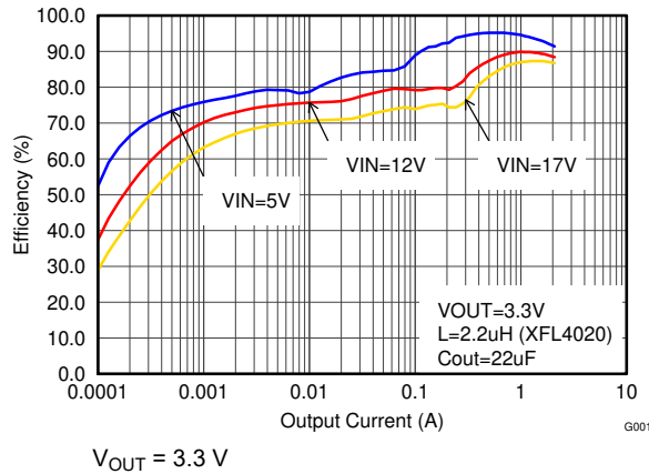
9-10. Efficiency With 2.5 MHz,
