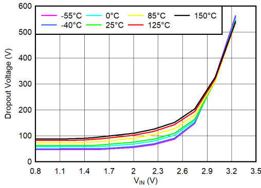
6-28. V IN Dropout Voltage vs V IN and Temperature (T J ) for I OUT = 1.5 A
