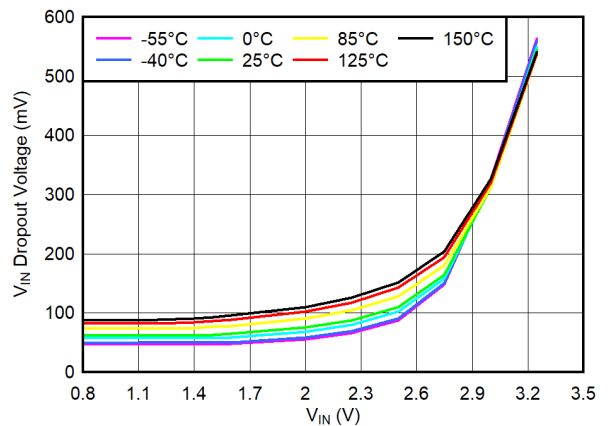
6-27. V IN Dropout Voltage vs V IN and Temperature (T J ) for I OUT = 500 mA
