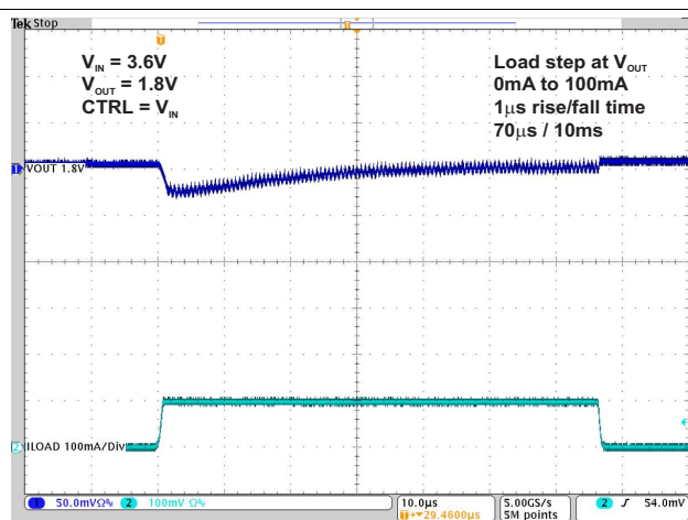
Figure 27. TPS82740A Load Transient Response V_{OUT} = 1.8V
