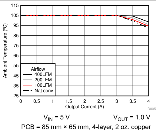
Figure 6-5. Safe Operating Area
