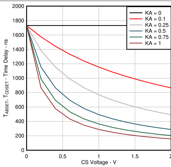
Figure 6-3. Delay Time set T_{ABSET} and T_{CDSET} (Over CS Voltage Variation and Selected K_A for R_{AB} and R_{CD} Equal 90 k \Omega )
