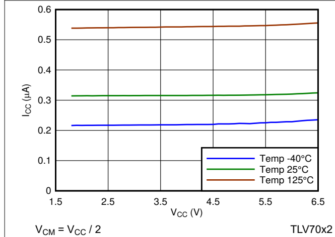
6-29. I_{CC} vs V_{CC}
