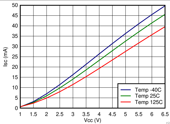
6-23. Output Short-Circuit (Source) Current vs Temperature
