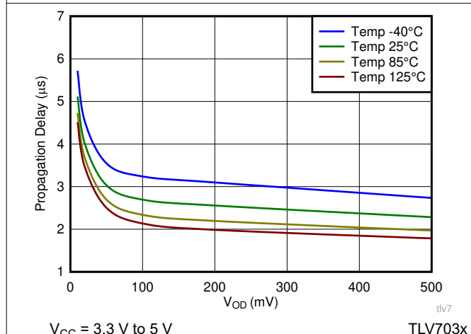
6-31. Propagation Delay (L-H) vs Input Overdrive
