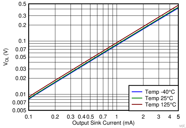
6-21. Output Voltage Low vs Output Sink Current
