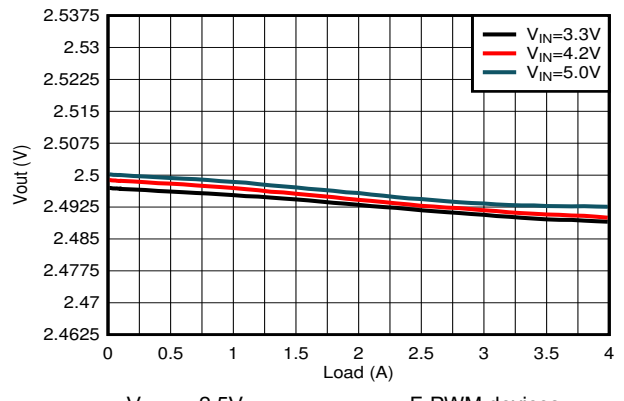
8-18. Load Regulation
