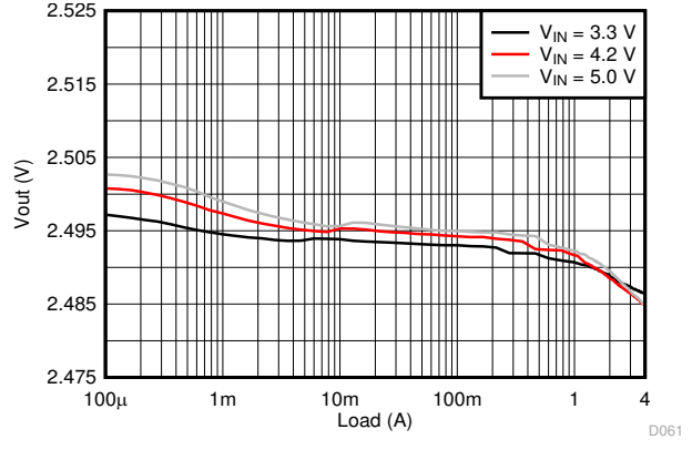
8-16. Load Regulation
