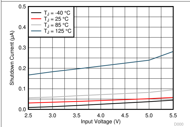
图 6-3. Shutdown Current
