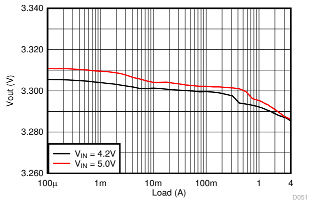
8-20. Load Regulation
