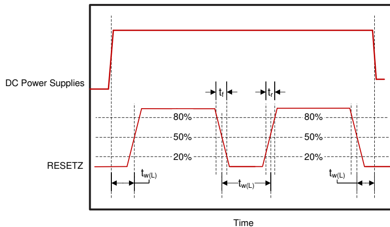
図 6-6. Power-Up and Power-Down RESETZ Timing
