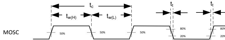
図 6-5. System Oscillators
