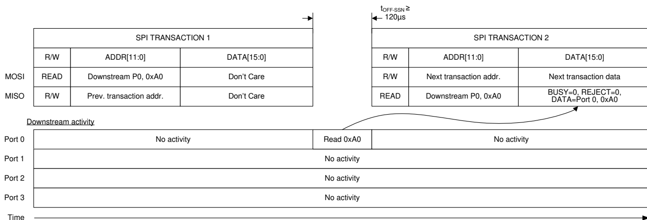
FIG 8-10. SPI Read Consisting of Two Separate SPI Transactions
