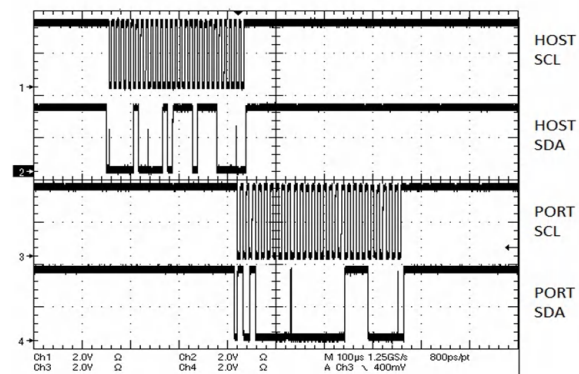
Figure 9-7. Scheduled Write Operation
