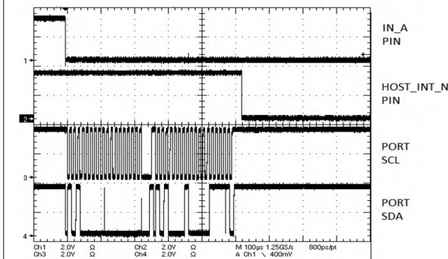
Figure 9-6. Interrupt-Driven Prefetch
