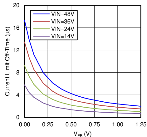
Figure 6-6. T OFF (I LIM ) vs V FB and V IN
