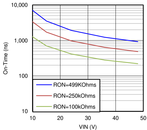
Figure 6-5. T ON versus V IN and R ON
