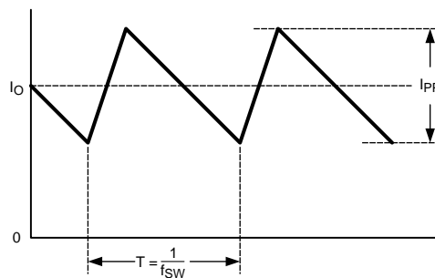
Figure 15. Inductor Current
