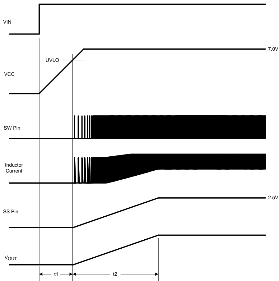
Figure 1. Start-Up Sequence
