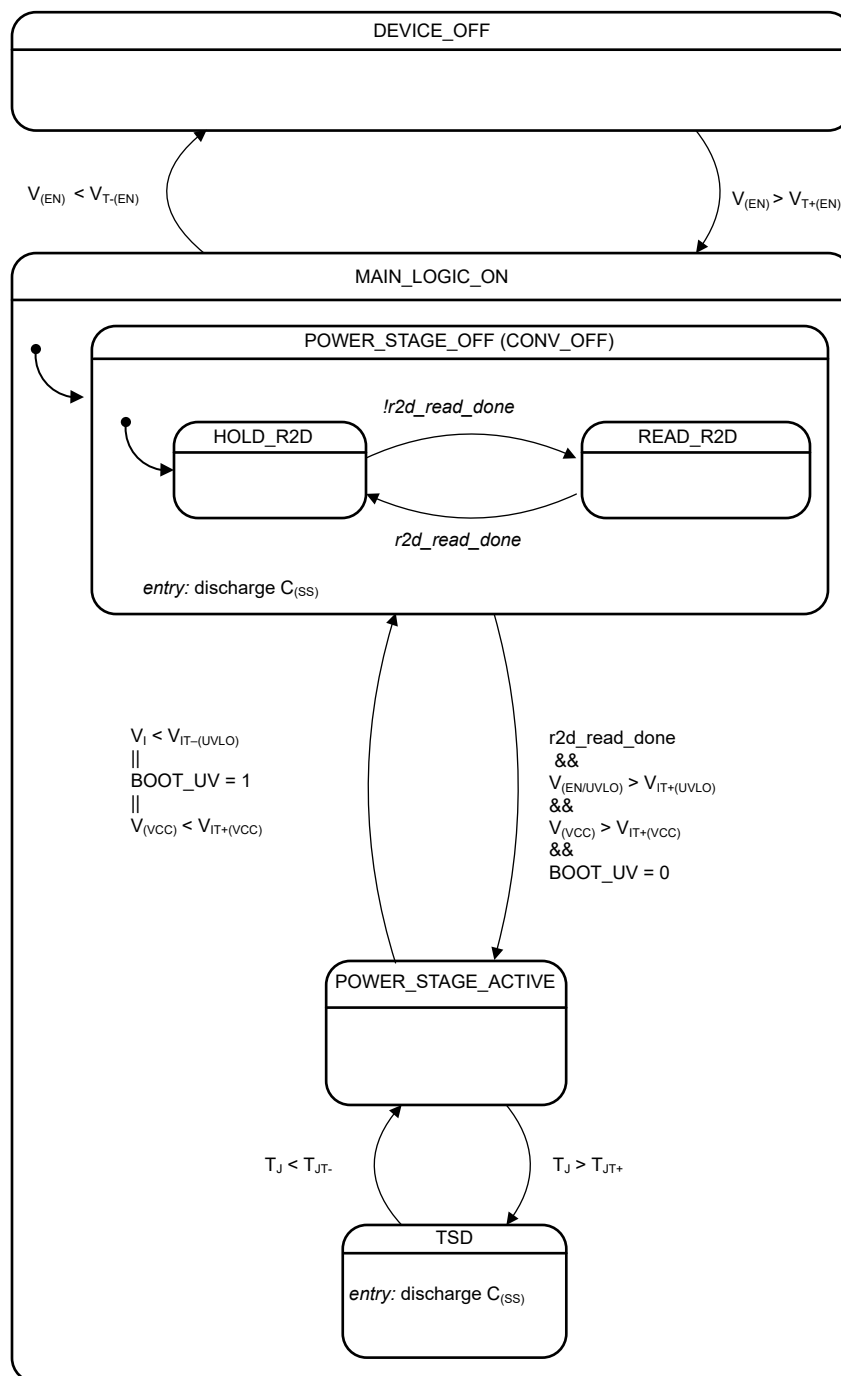
図 8-29. State Diagram
