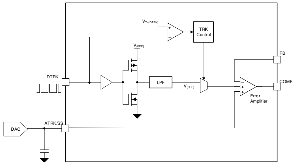
图 8-21. Output Voltage Tracking Functional Block Diagram
