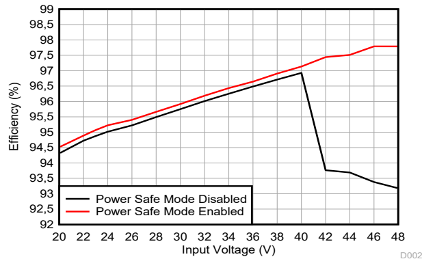
図 10-6. Efficiency Versus V_I ( V_O = 48V, I_O = 5A)
