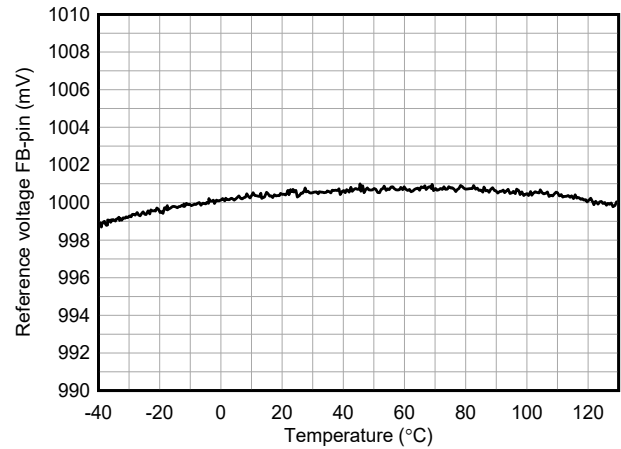
FIG 6-4. FB Pin Reference Voltage versus Temperature
