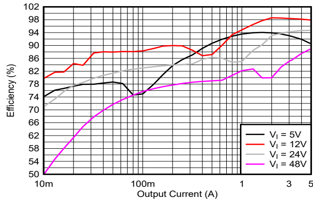
図 10-2. Efficiency Versus I_O (MODE = 0V V_O = 12V)
