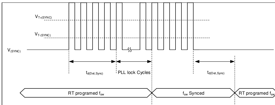
8-20. Timing Diagram SYNC Function
