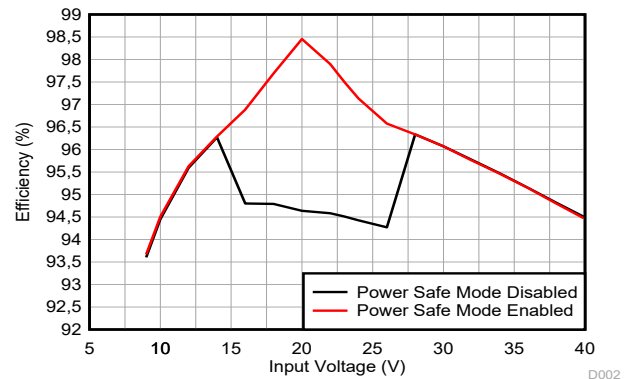
図 10-5. Efficiency Versus V_I ( V_O = 20V, I_O = 5A)
