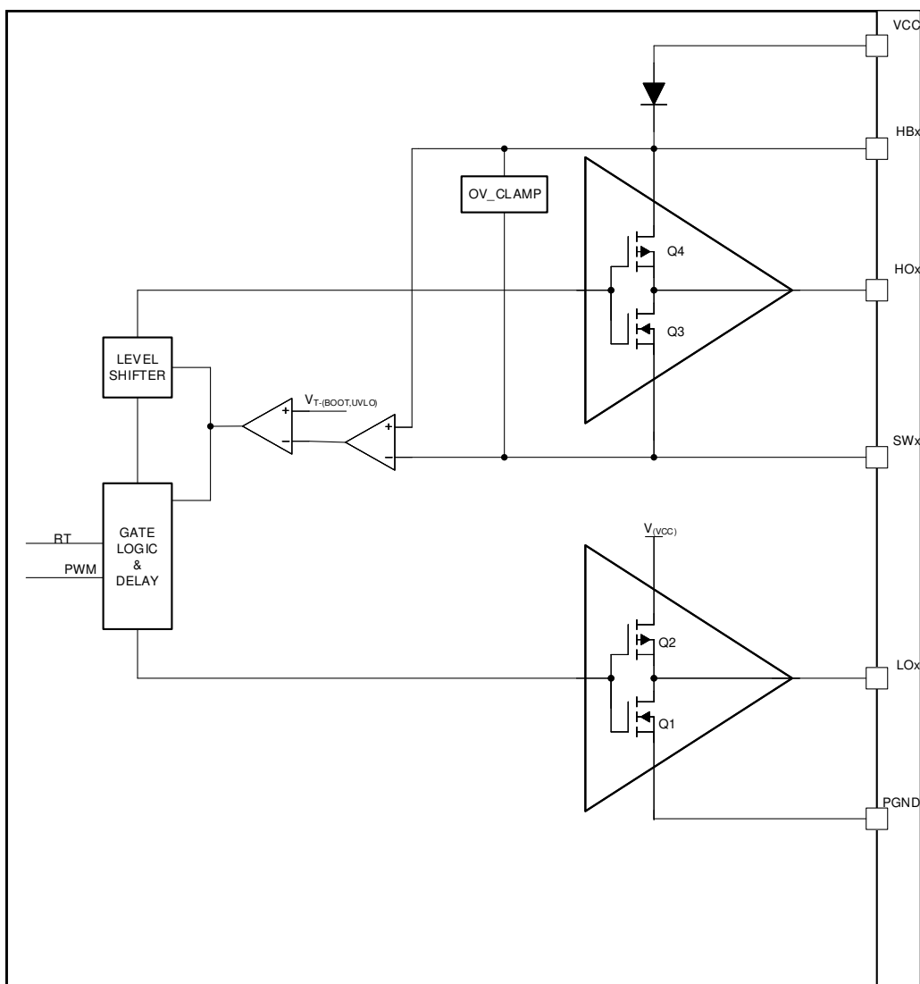
図 8-24. Functional Block Diagram Gate Driver
