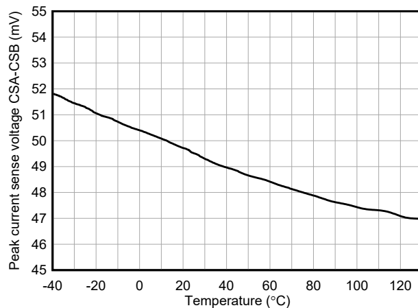
FIG 6-5. Current Limit Threshold Voltage Versus Temperature
