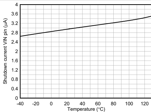
FIG 6-7. Shutdown Current into VIN versus Temperature V_{EN/UVLO} = 0\text{V} , V_{(VIN)} = 12\text{V} , V_{(BIAS)} = 0\text{V}
