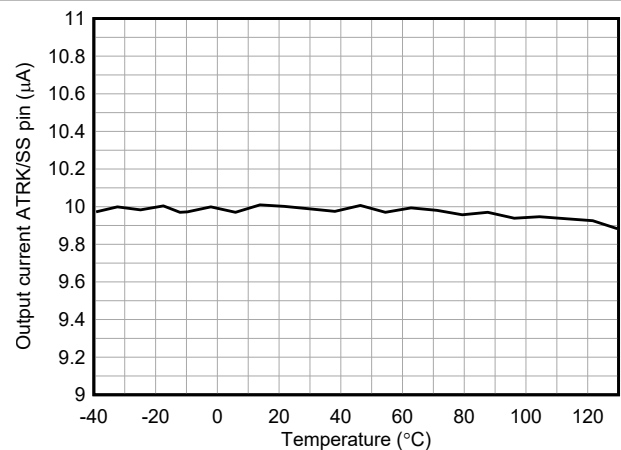
FIG 6-8. Soft-Start current versus Temperature
