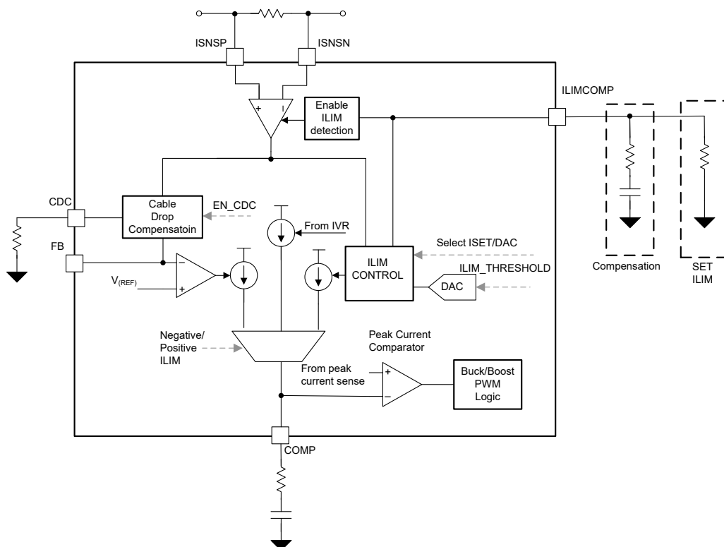
8-16. Current Monitor Functional Block Diagram
