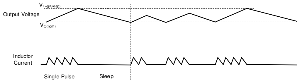
図 8-6. Timing Diagram for the Power Save Mode
