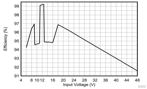
図 10-7. Efficiency Versus V_I ( V_{(PCM,low)} = 11V, V_{(PCM,high)} = 13V, I_O = 5A, MODE = VCC2)
