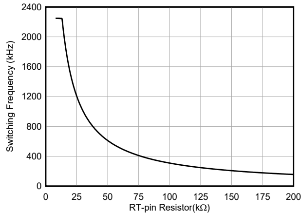
FIG 6-3. Switching Frequency Versus RT Resistance
