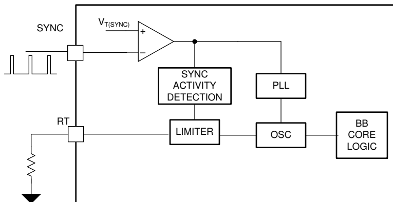
8-19. Main Oscillator Functional Block Diagram
