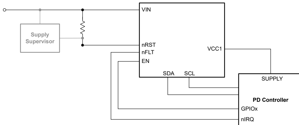
図 8-13. Simplified Schematic
