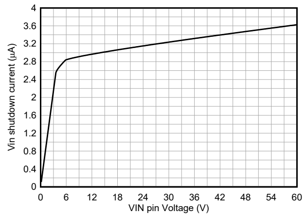
FIG 6-6. Shutdown Current into VIN versus Pin Voltage V_{EN/UVLO} = 0\text{V} , V_{(VIN)} = 12\text{V} , V_{(BIAS)} = 0\text{V}
