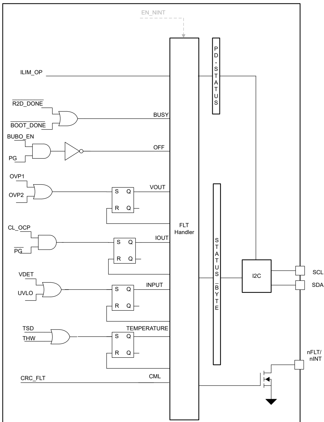
8-26. Functional Block Diagram Fault Handler
