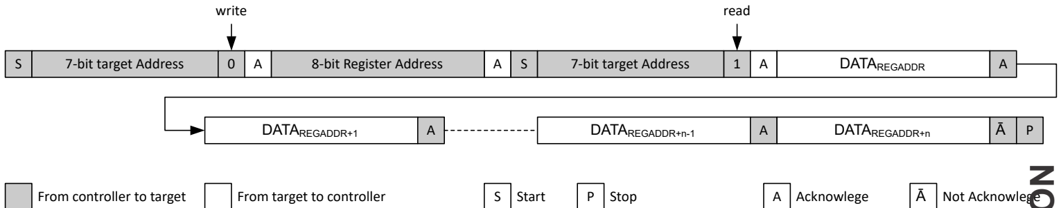
8-34. Sequential READ starting from a defined register address
