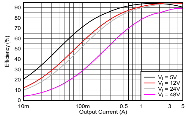
図 10-3. Efficiency Versus I_O (MODE = VCC2 V_O = 12V)
