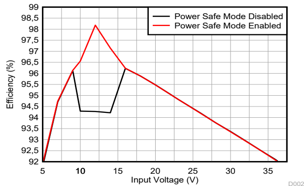
図 10-4. Efficiency Versus V_I ( V_O = 12V, I_O = 5A)
