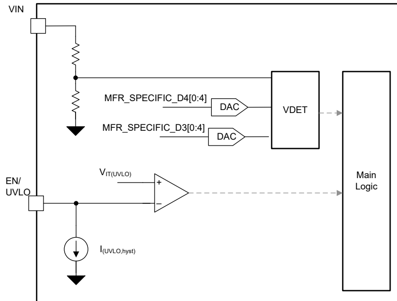
図 8-12. Functional Block Diagram UVLO and VDET
