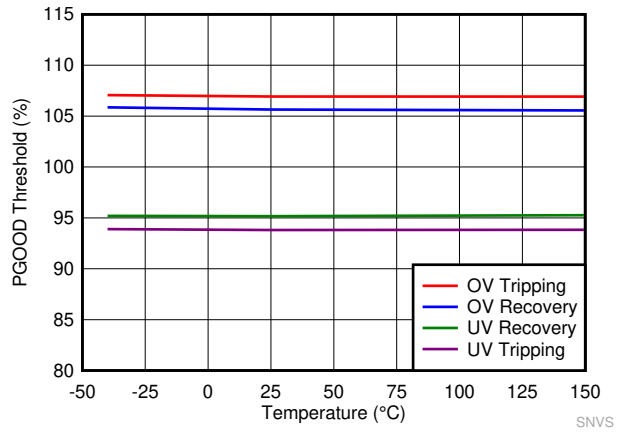
7-7. PGOOD Thresholds
