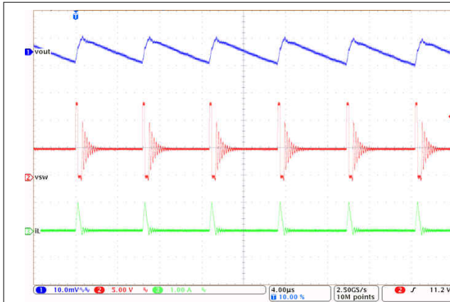
Figure 9-28. LM61430-Q1 Switching Waveform and V_{OUT} Ripple
