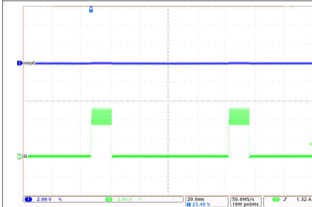
Figure 9-34. LM61430-Q1 Short Circuit Protection
