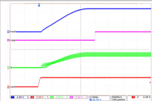
Figure 9-33. LM61430-Q1 Start-up with 3 A
