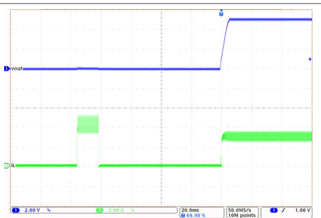
8-13. Short-Circuit Recovery
