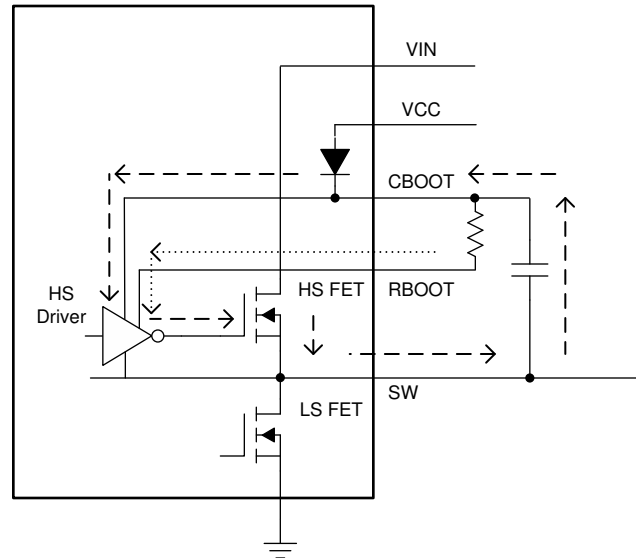
8-7. Simplified Circuit Showing How RBOOT Functions
