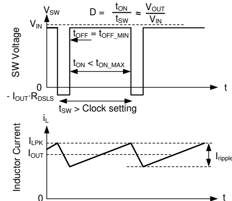
8-19. Frequency and Output Voltage in Dropout
