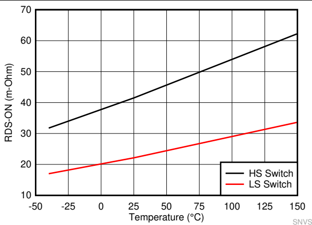
7-5. High-Side and Low-Side Switches R_{\text{DS\_ON}}
