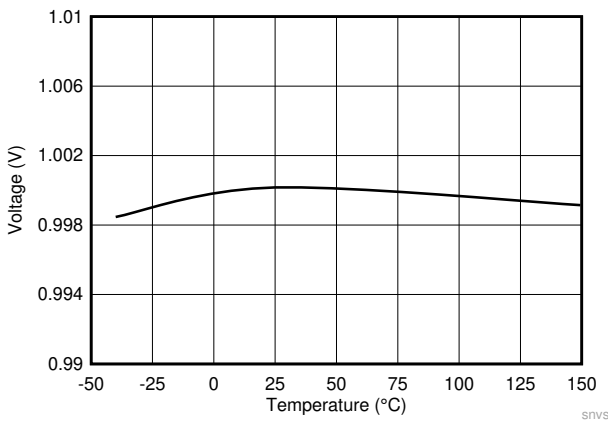
7-3. Feedback Voltage
