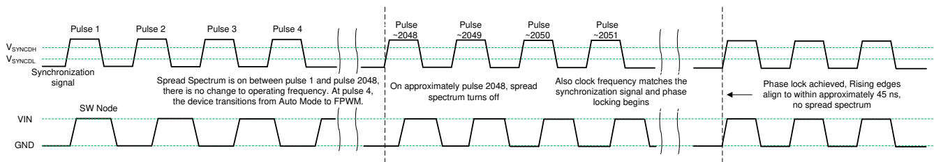
8-4. Synchronization Process
