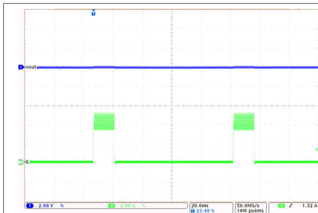
8-12. Inductor Current Bursts During Hiccup
