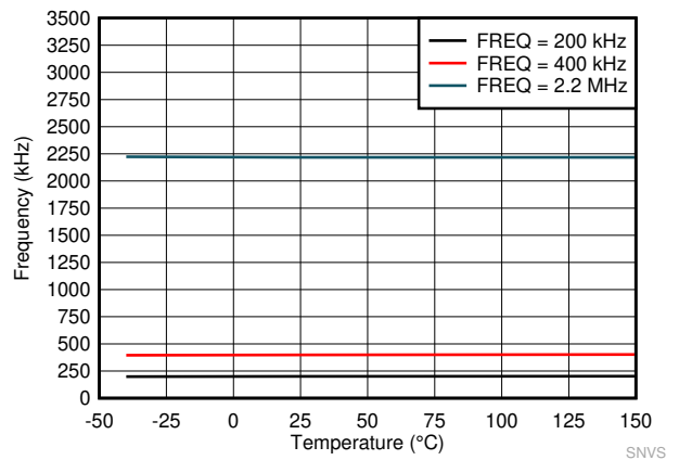
7-4. Switching Frequency Set by RT Resistor
