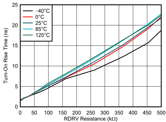
FIG 7-3. Turn-On Rise Time vs Drive Strength Resistance
