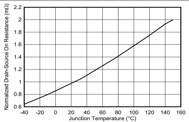
FIG 7-6. Normalized On-Resistance vs Junction Temperature
