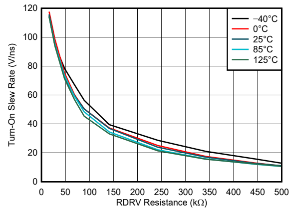
FIG 7-4. Turn-On Slew Rate vs Drive Strength Resistance
