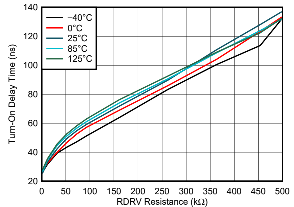
FIG 7-2. Turn-On Delay Time vs Drive Strength Resistance
