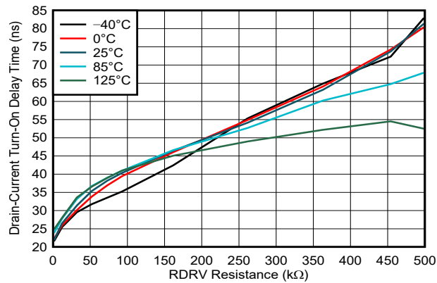
FIG 7-1. Drain-Current Turn-On Delay Time vs Drive Strength Resistance
