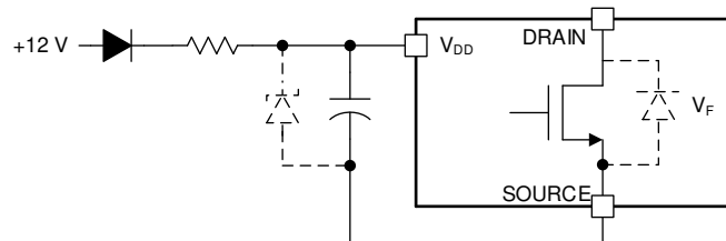
11-2. Suggested Bootstrap Regulation Circuit
