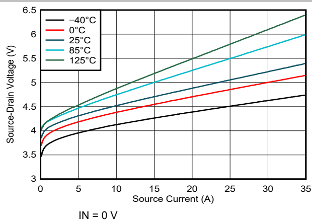
FIG 7-5. Off-State Source-Drain Voltage vs Source Current
