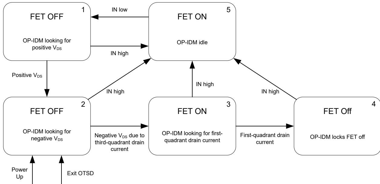
FIG 9-4. Operational Ideal-Diode Mode (OP-IDM) State Machine
