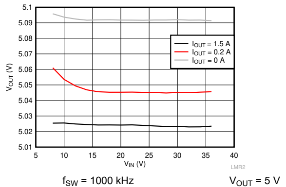
Figure 6-6. Line Regulation
