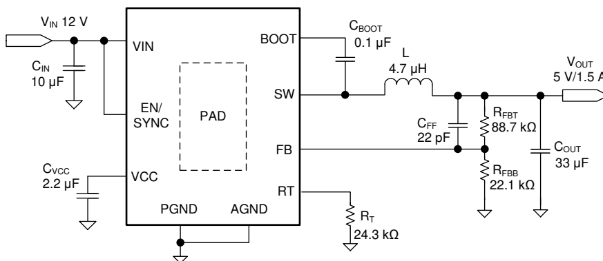
図 8-1. Application Circuit
