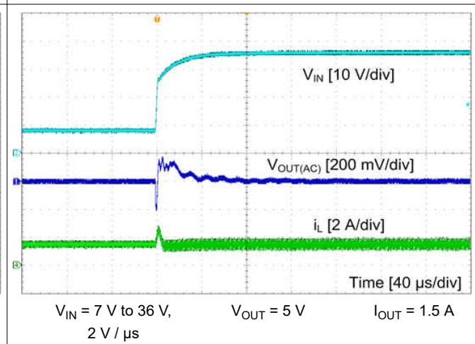
8-7. Line Transient
