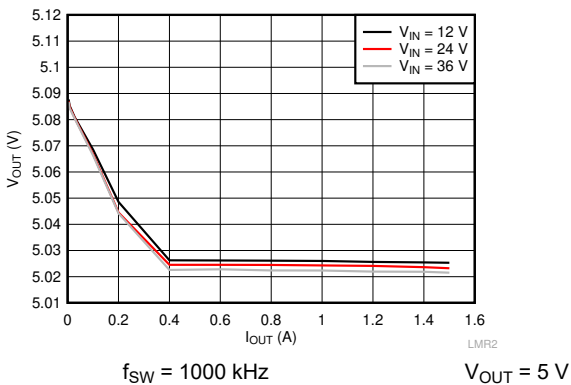
Figure 6-5. Load Regulation
