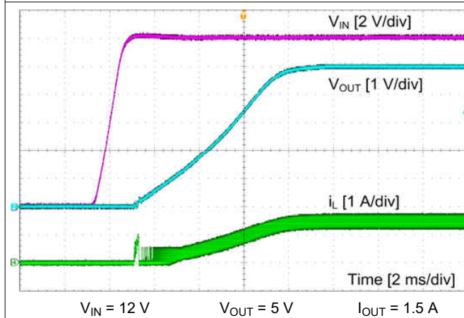
8-4. Start-Up by V_{IN}
